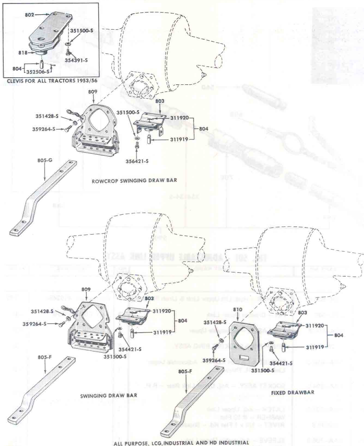
FIG. 5E1 - SWINGING DRAWBAR & RELATED PARTS
