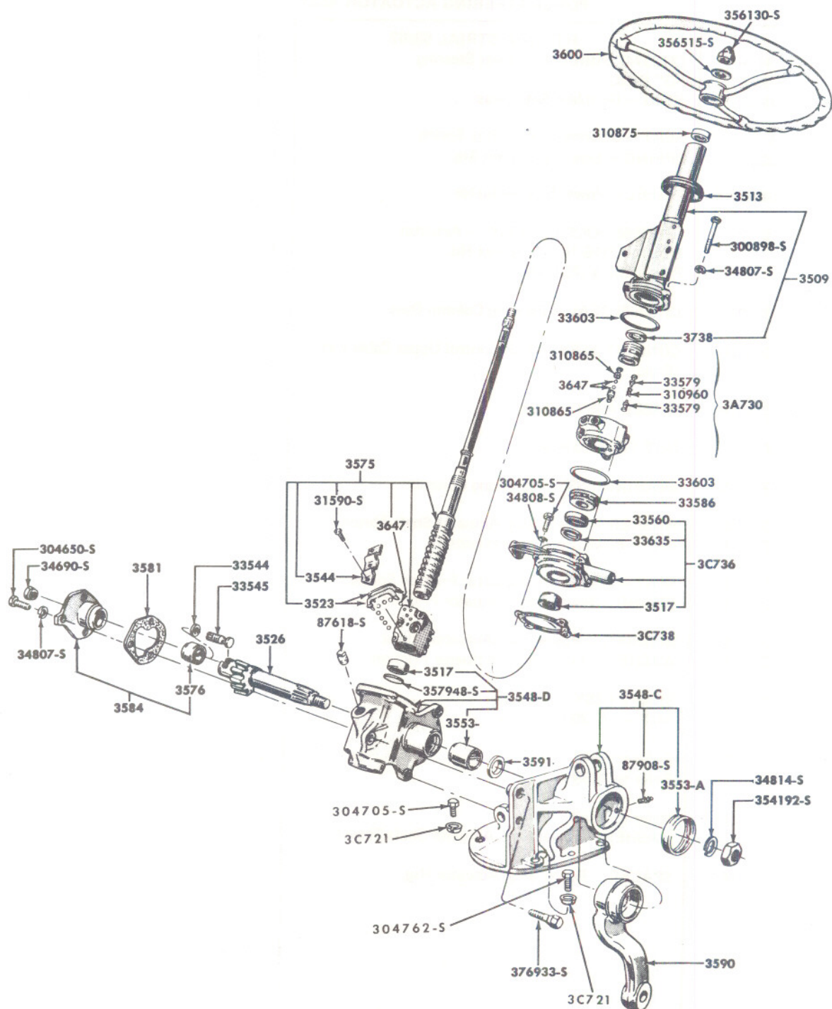
FIG. 3B5 - H D INDUSTRIAL STEERING GEAR ASSY.
