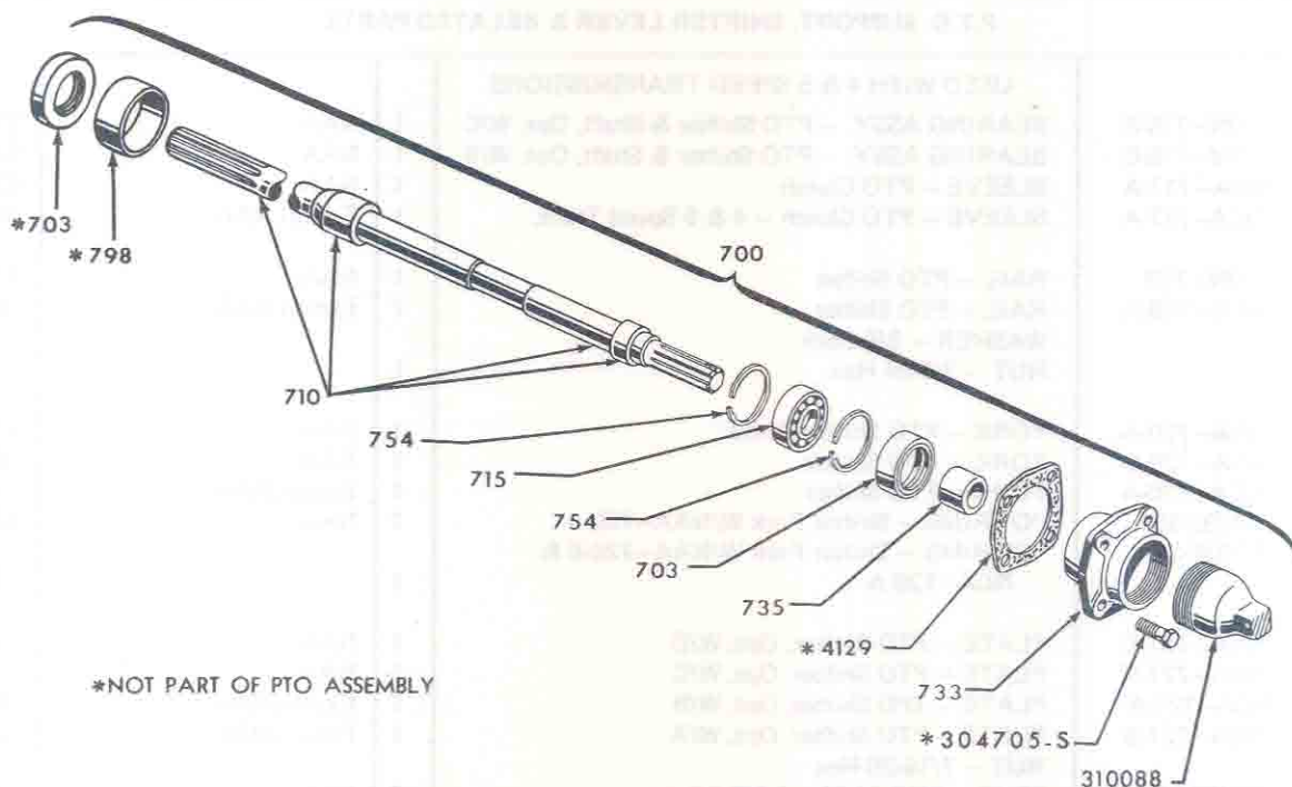
FIG. 7E2 - 1 1/8" P.T.O. ASSEMBLY & RELATED PARTS 1953/56
