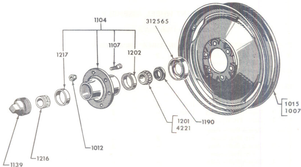
FIG. 1A2 - HEAVY DUTY FRONT WHEEL ASSY.
