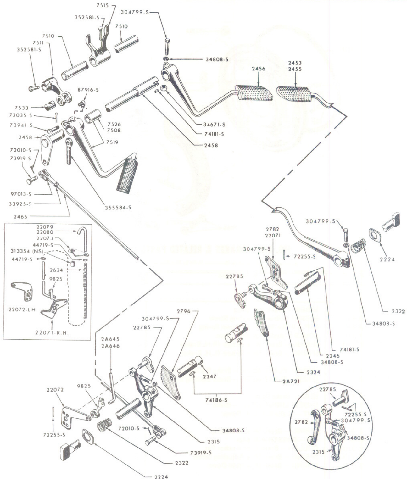
FIG. 2B1 - BRAKE & CLUTCH CONTROLS 53/57
