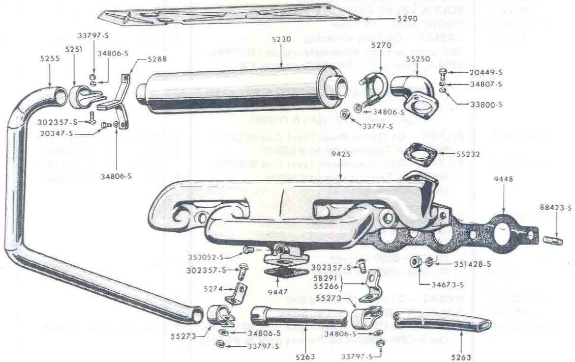
FIG. 6E2 - HORIZONTAL EXHAUST SYSTEM
