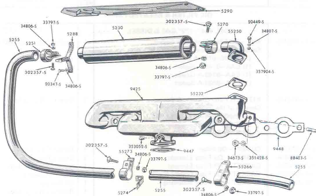
FIG. 6E1 - HORIZONTAL EXHAUST SYSTEM 53/54
