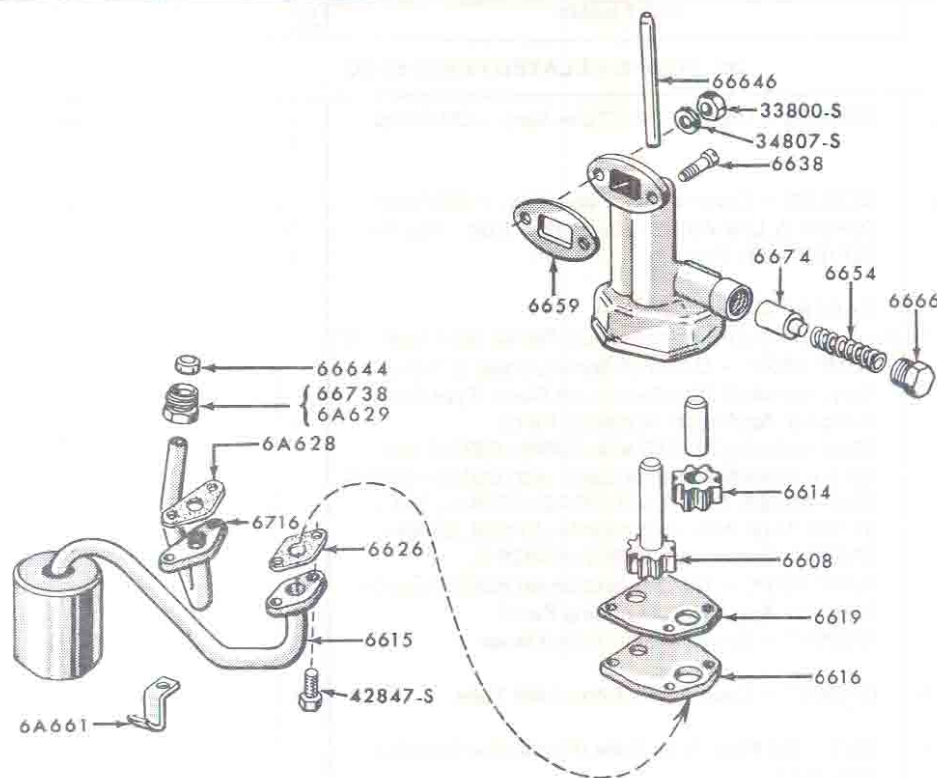
FIG. 6C1 OIL PUMP & RELATED PARTS 53/60
