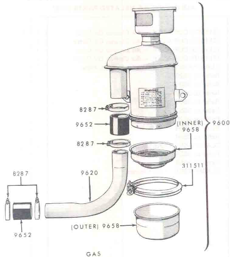
FIG. 9C3 GASOLINE AIR CLEANER & RELATED PARTS 1958/
