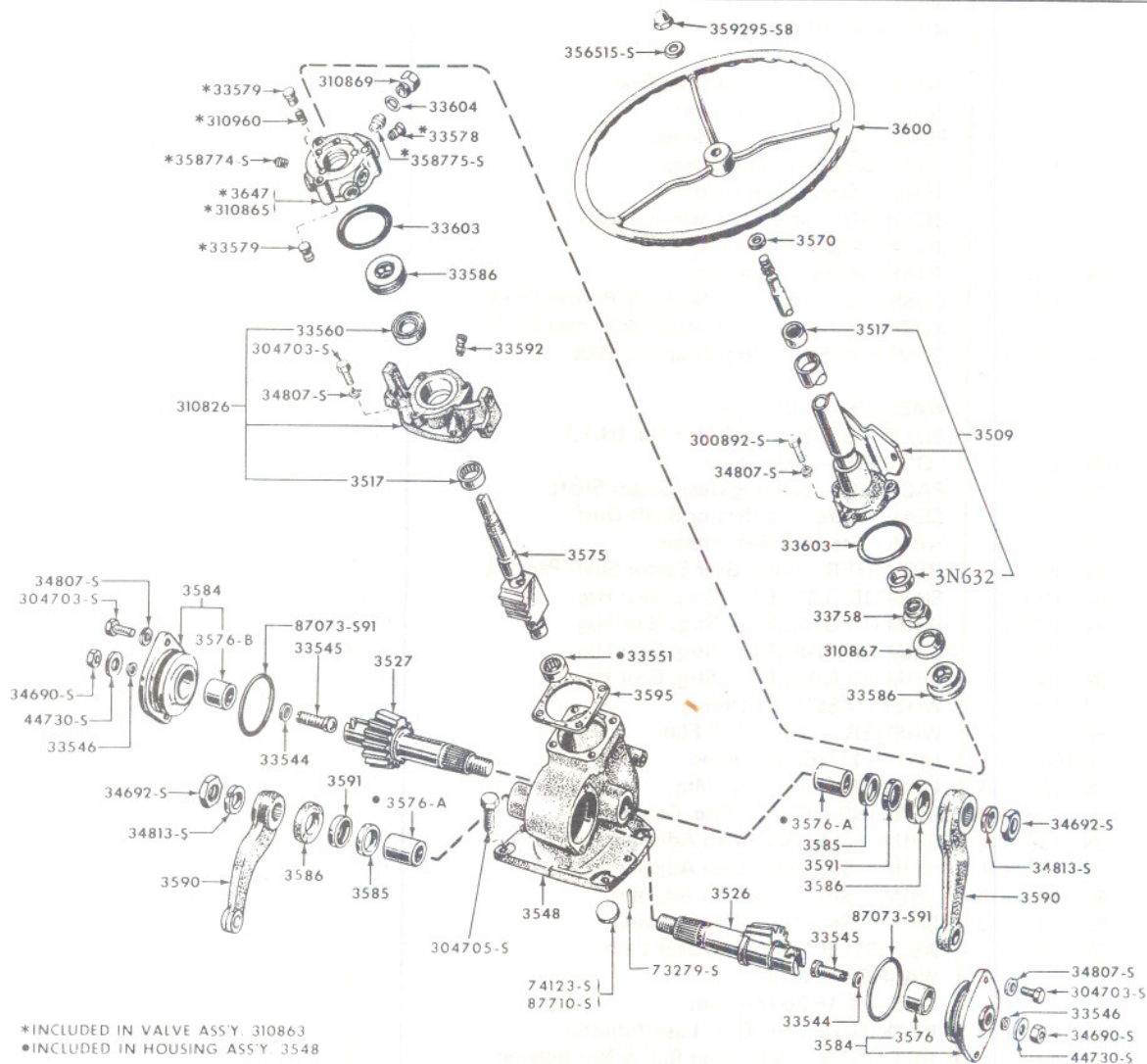
FIG. 3B2 - POWER STEERING GEAR & RELATED PARTS
