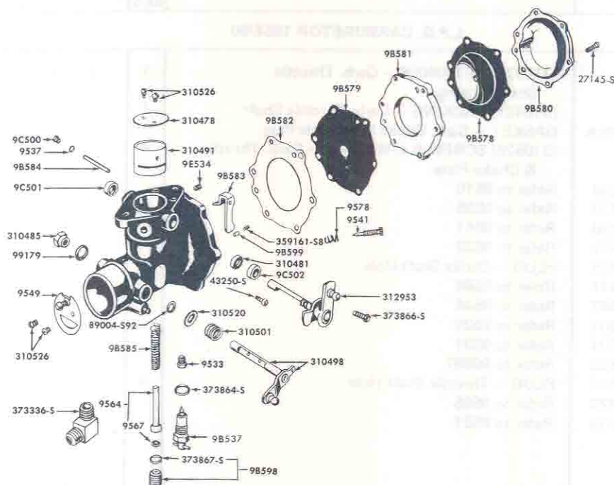
FIG. 9B4 - L.P.G. CARBURETOR ASSY. - 1961/
