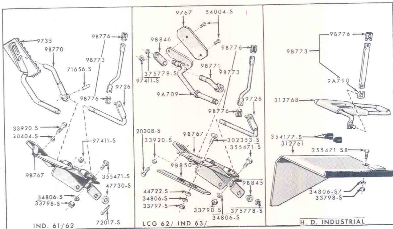
FIG. 9D4 - THROTTLE & ACCELERATOR CONTROLS (DIESEL) INDUSTRIAL, 61/—L.C.G., 62/—H.D. INDUSTRIAL, 63/
