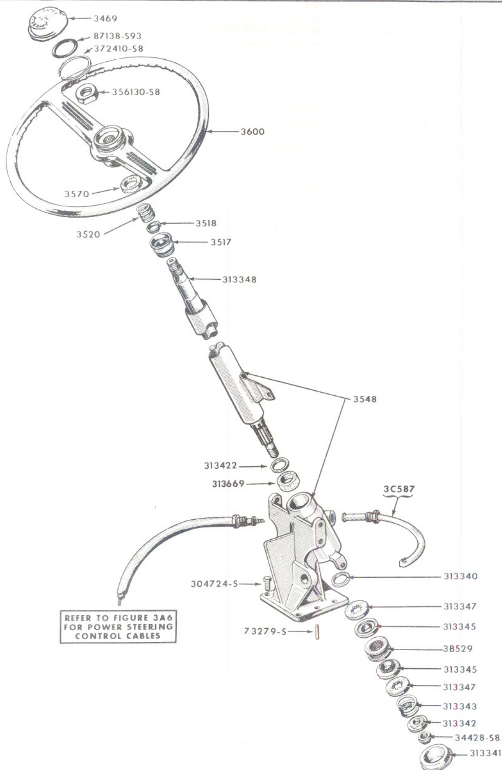
FIG. 3B4 - POWER STEERING ACTUATOR ASSY.
