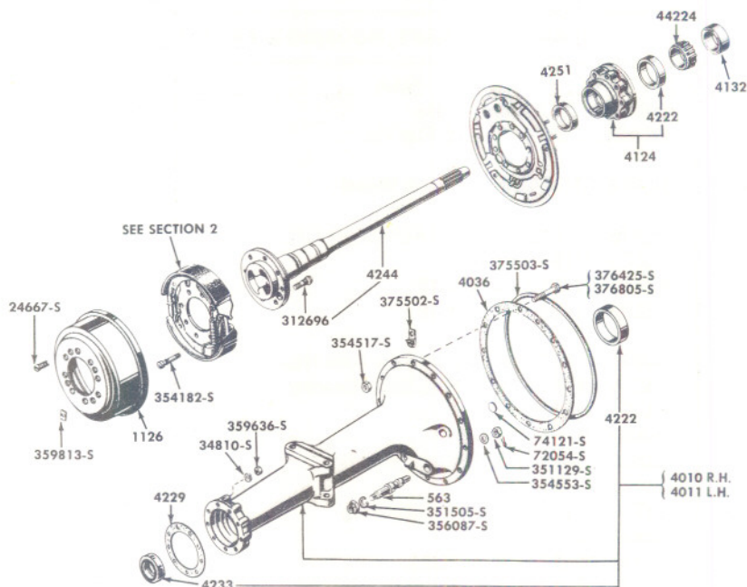
FIG. 4A2 - REAR AXLE SHAFT, HOUSING & RELATED PARTS 55/
