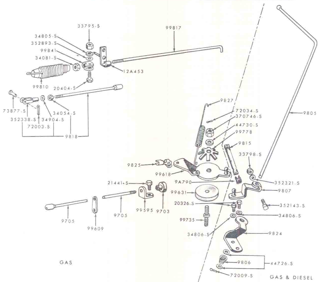
FIG. 9D1 - THROTTLE CONTROLS & RELATED PARTS, 1953/
