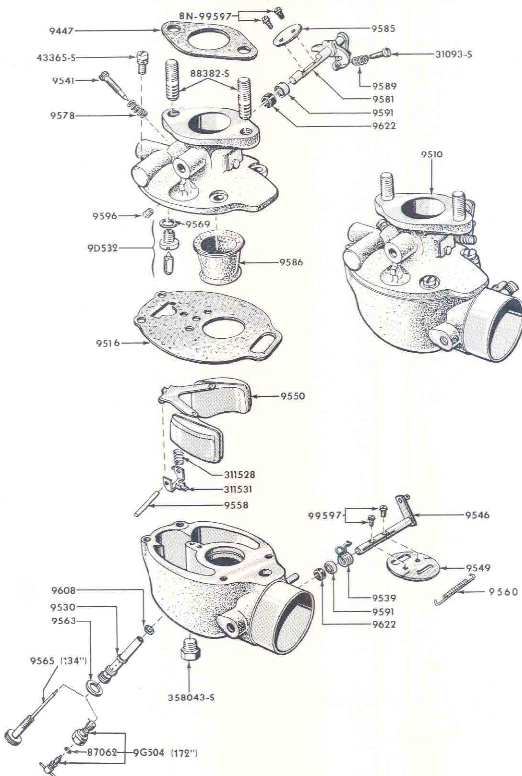
FIG. 9B2 - CARBURETOR ASSY. - 1958/
