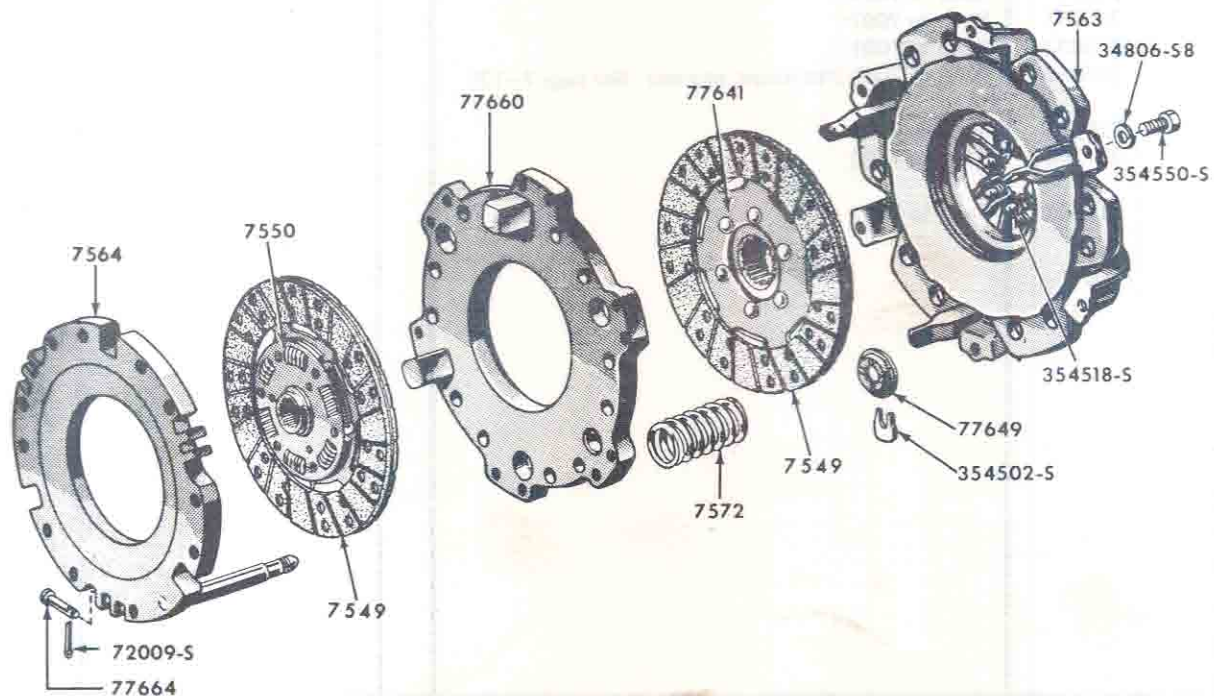
FIG. 7C2 - DOUBLE CLUTCH ASSEMBLY
