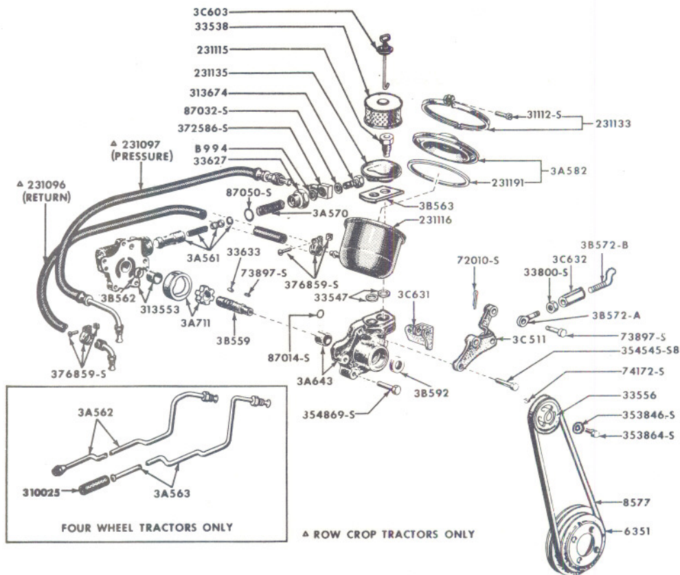
FIG. 3C3 POWER STEERING PUMP, OIL RESERVOIR & RELATED PARTS 1959/
