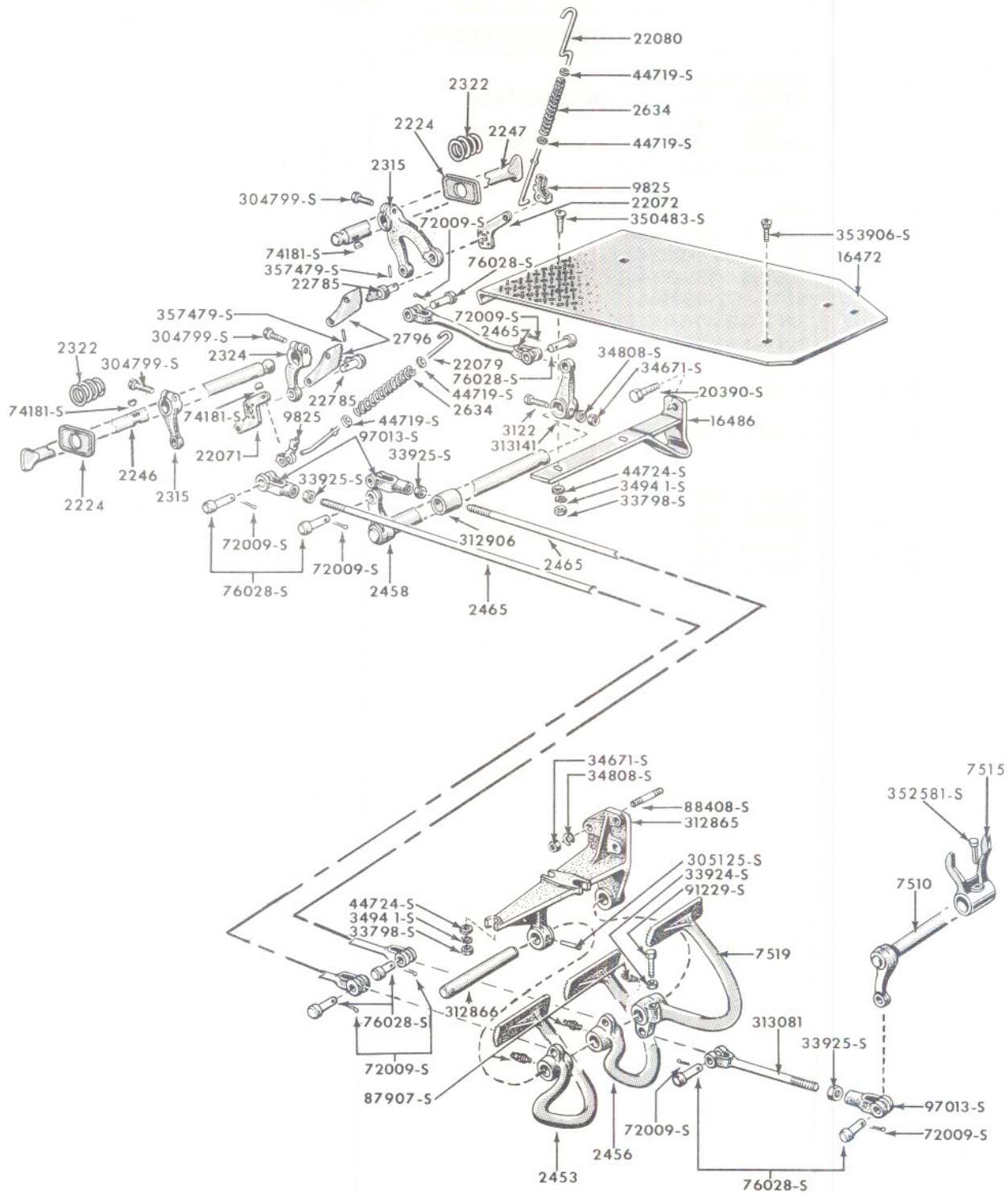
FIG. 2C1- BRAKE & CLUTCH CONTROLS (OFFSET)
