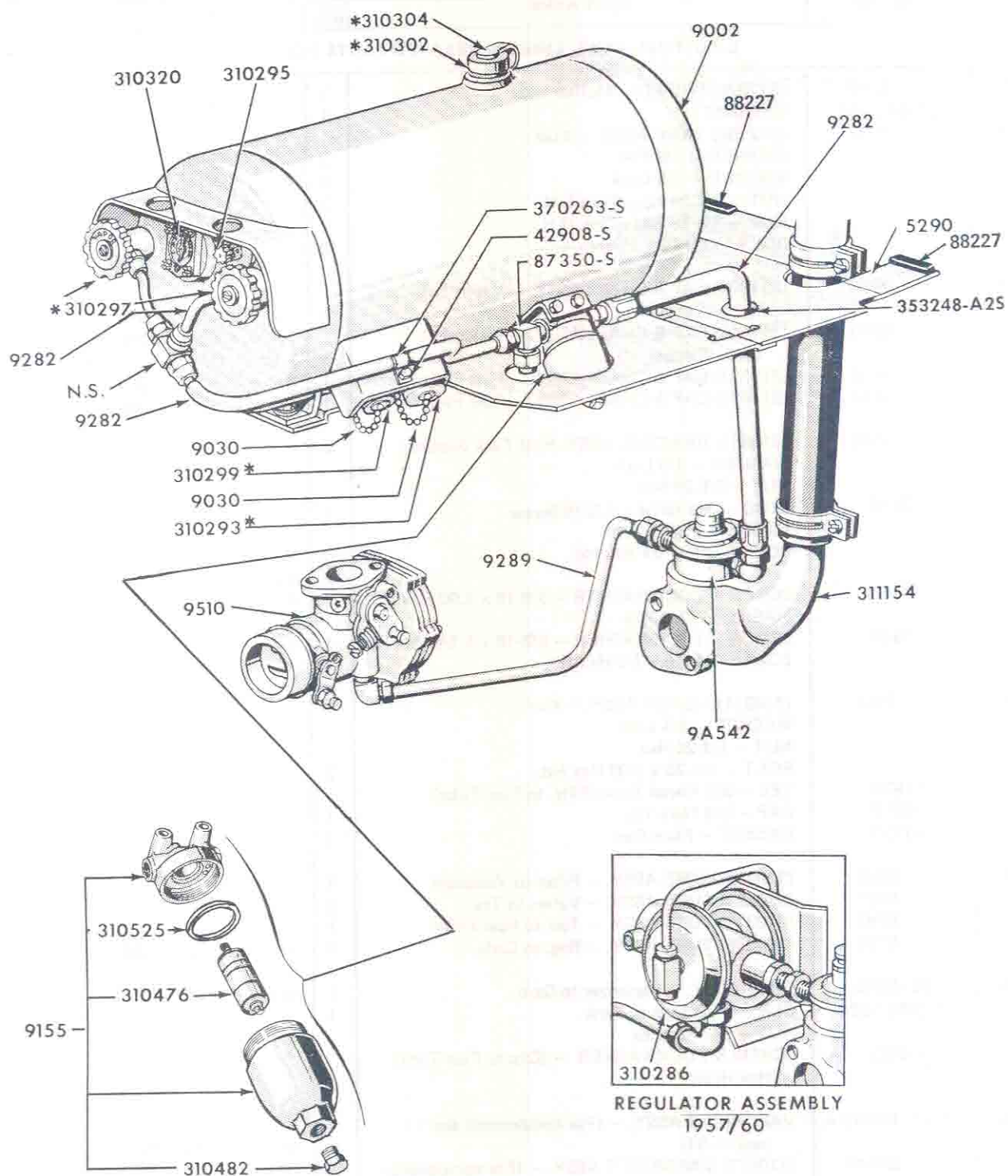
FIG. 9A2 L.P.G. FUEL TANK, LINES & RELATED PARTS 1957/
