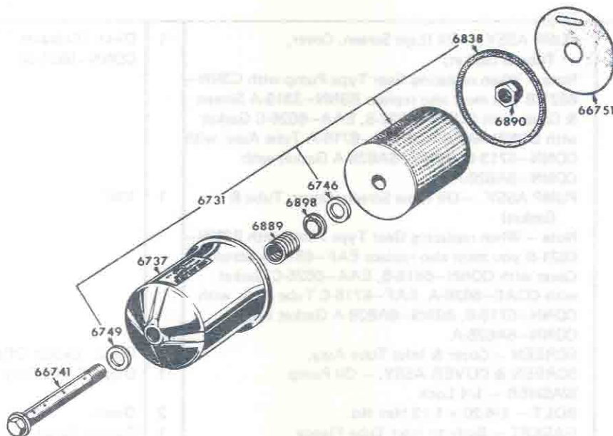
FIG. 6D1 - OIL FILTER & RELATED PARTS
