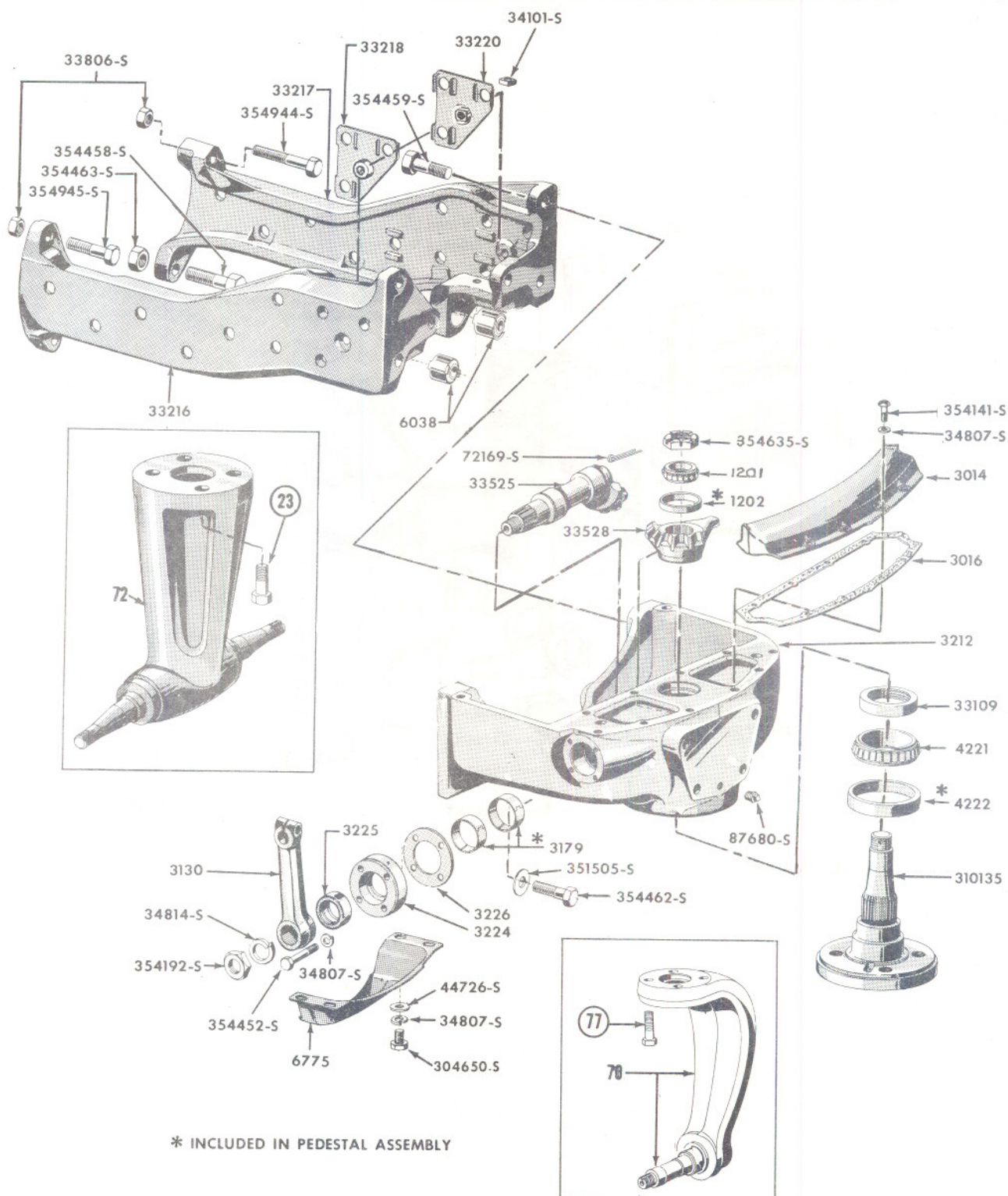
FIG. 3A4B2 - ROWCROP FRONT PEDESTAL & RELATED PARTS 1957/
