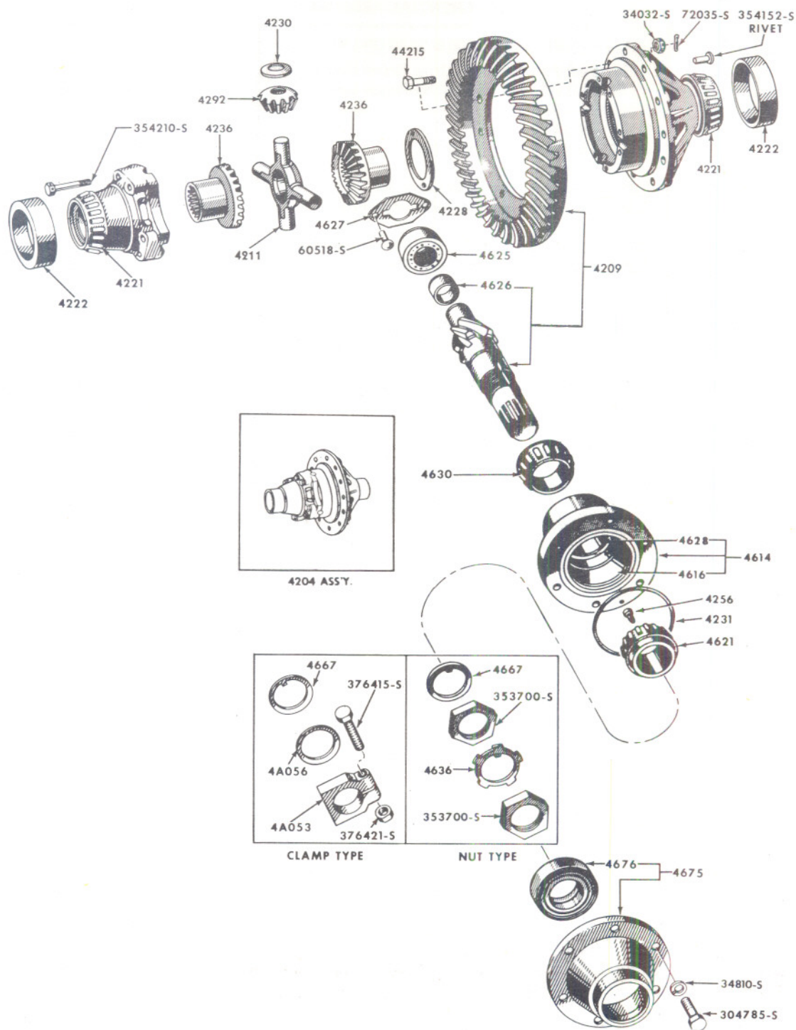
FIG. 4C2 - DIFFERENTIAL ASSEMBLY
