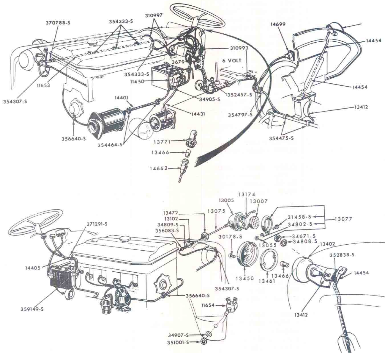
FIG. 11A4 - LIGHTING & WIRING 1958/
