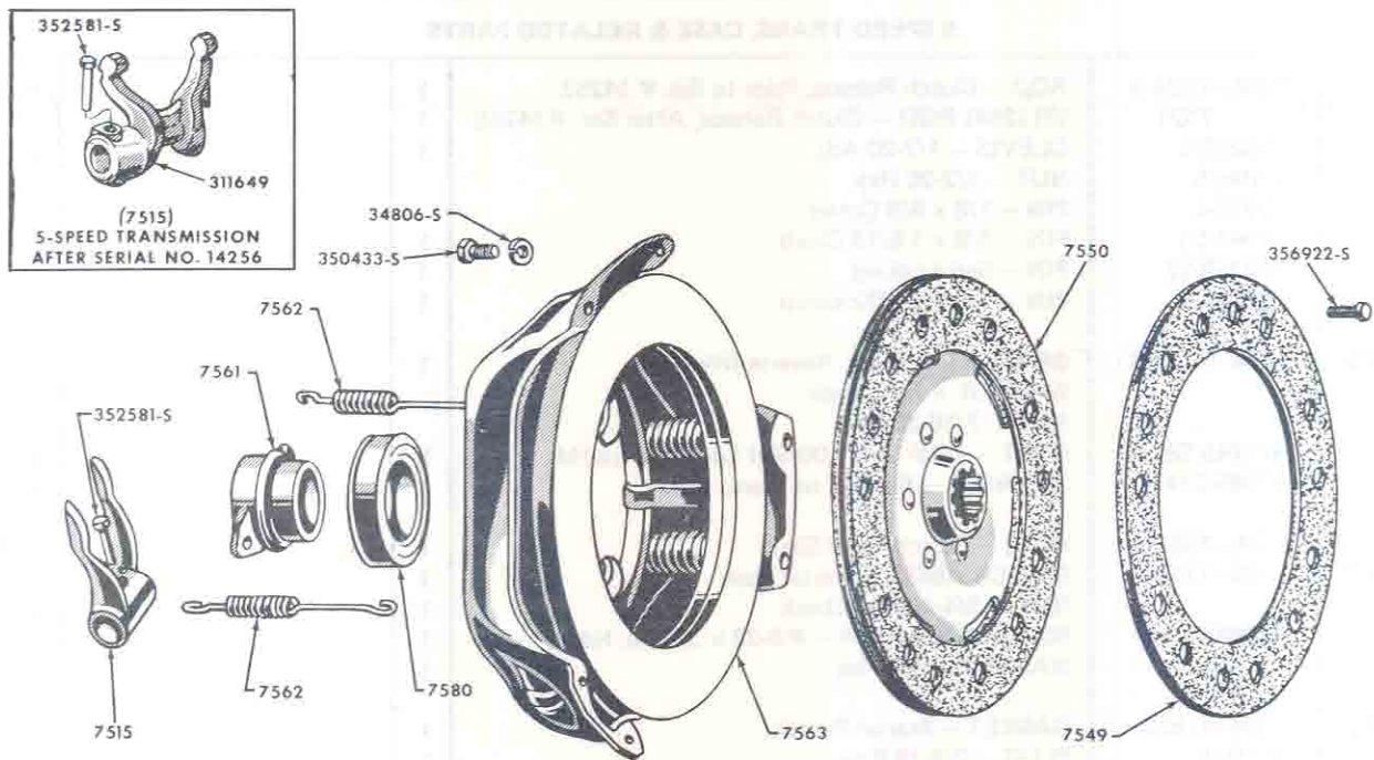
FIG. 7C1 - SINGLE CLUTCH ASSEMBLY
