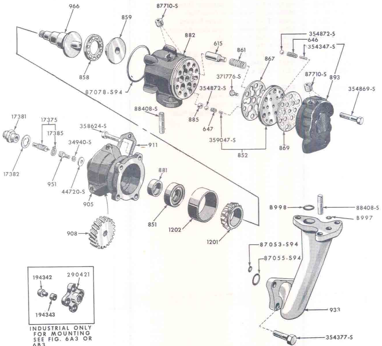
FIG. 10A3 - HYDRAULIC PUMP - PISTON TYPE 1953/ 10-8
