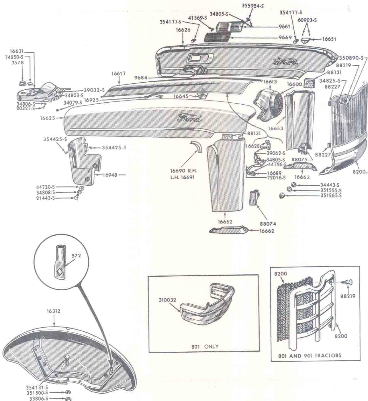
FIG. 14B1 - SHEET METAL & RELATED PARTS 1953/62
