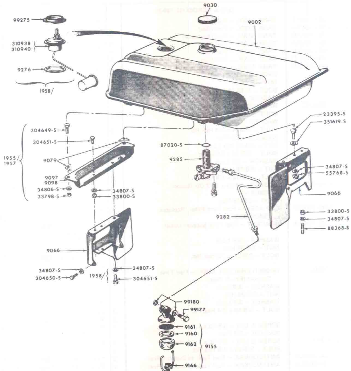
FIG. 9A1B - FUEL TANK LINES & RELATED PARTS GAS 1955/
