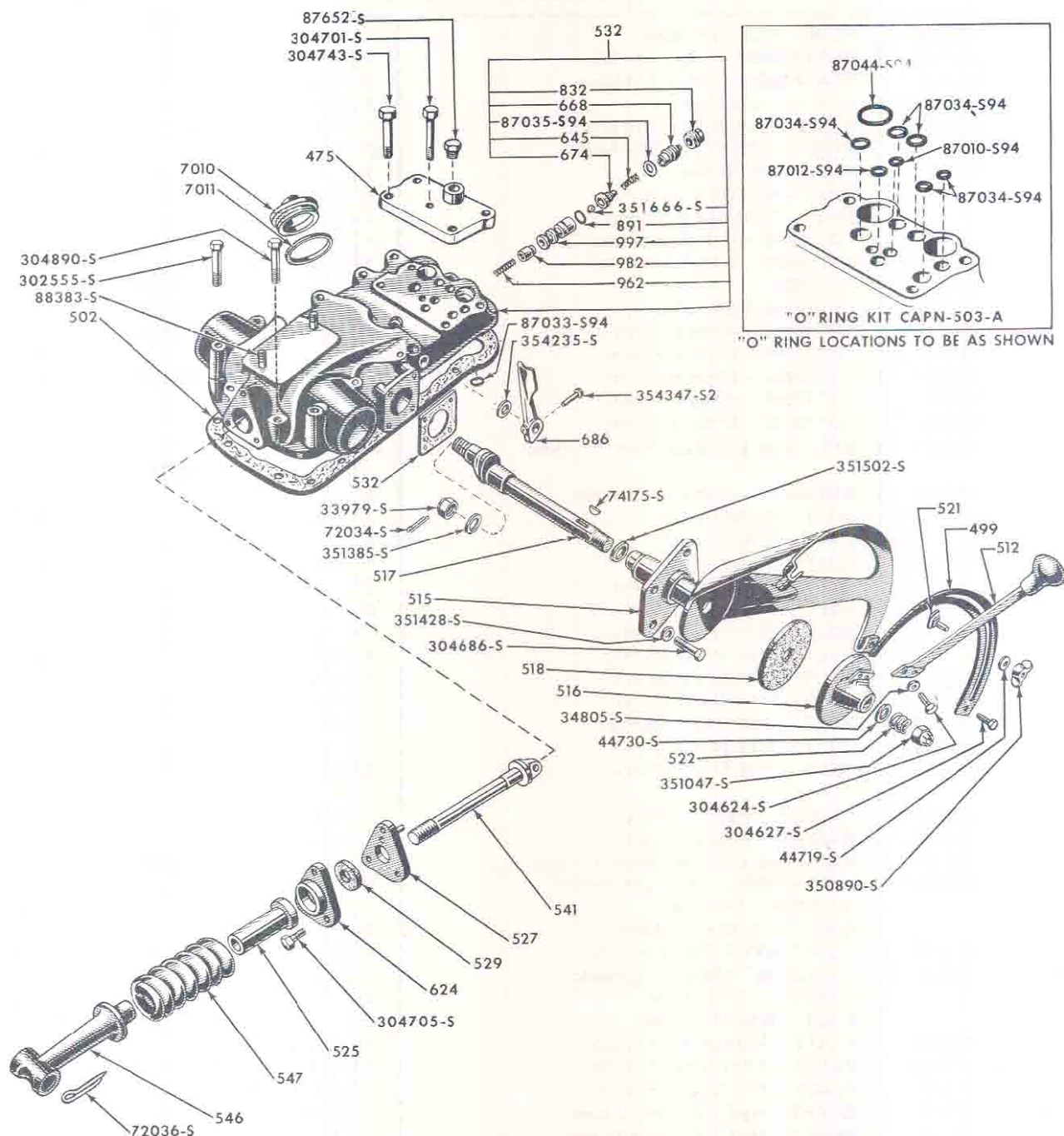
FIG. 5A2 - HYDRAULIC LIFT COVER & RELATED PARTS 1955/
