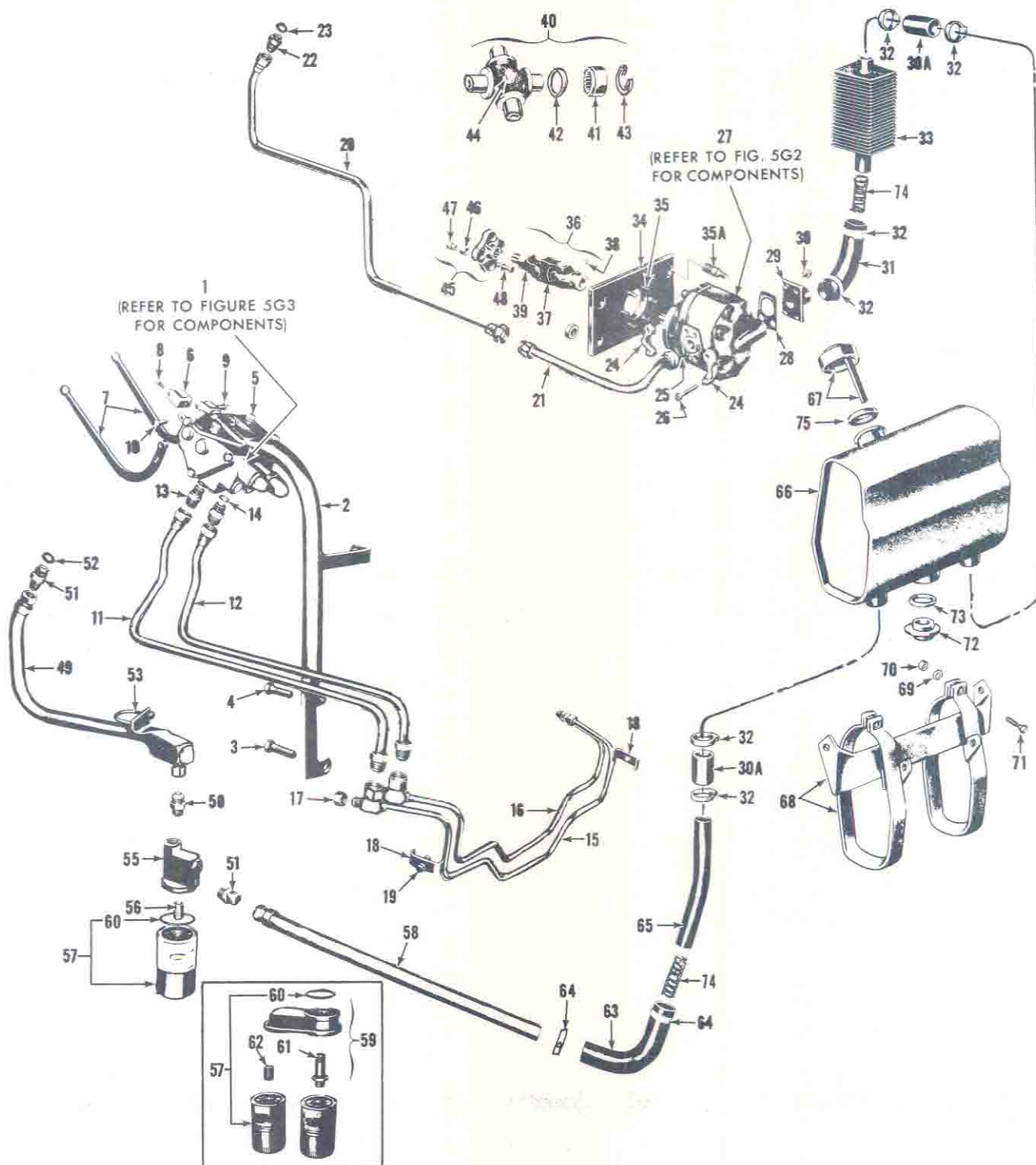
FIG. 5G1 - H.D. INDUSTRIAL HYDRAULIC PACKAGE
