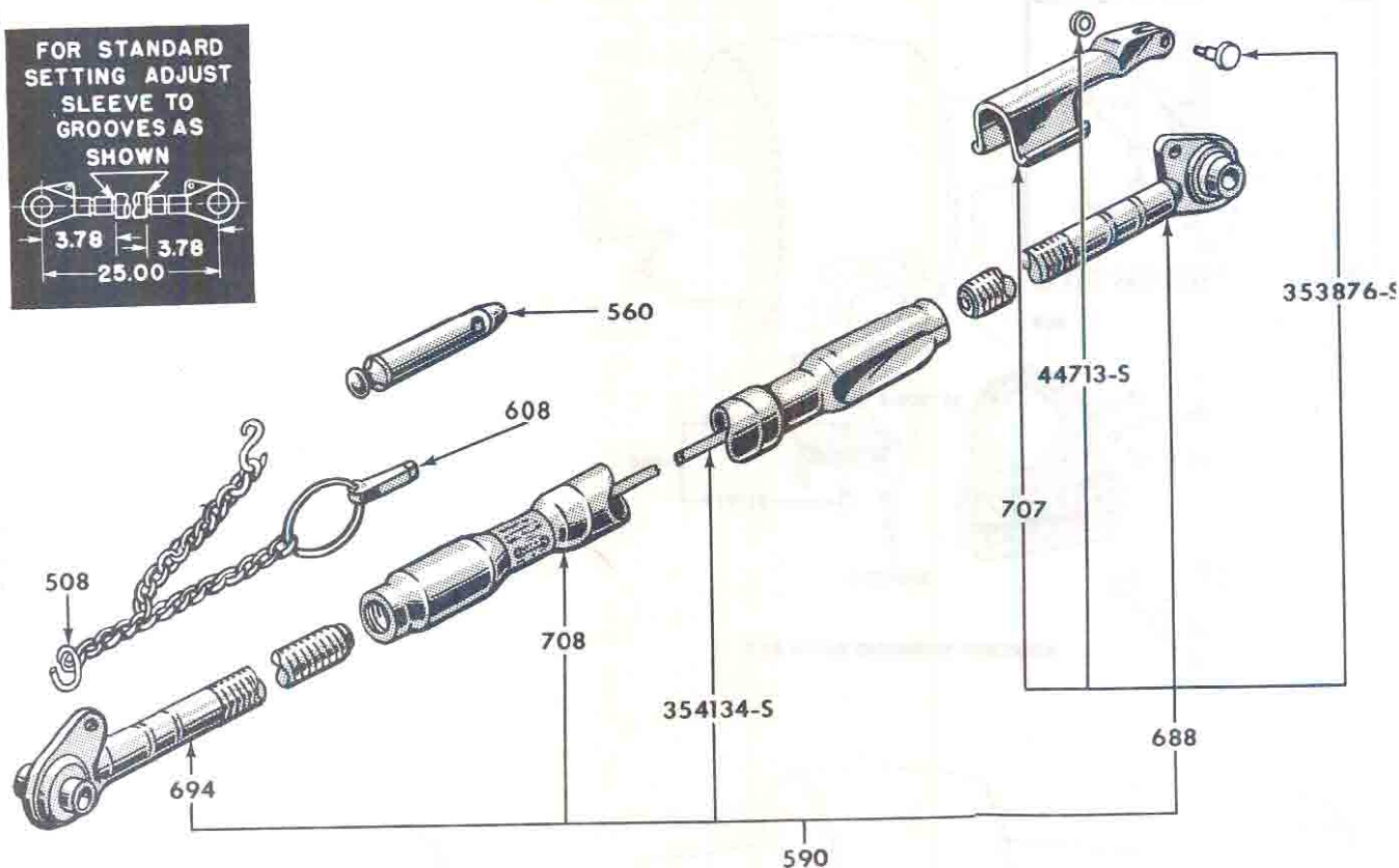
FIG. 5D1 - ADJUSTABLE UPPER LINK ASSY.
