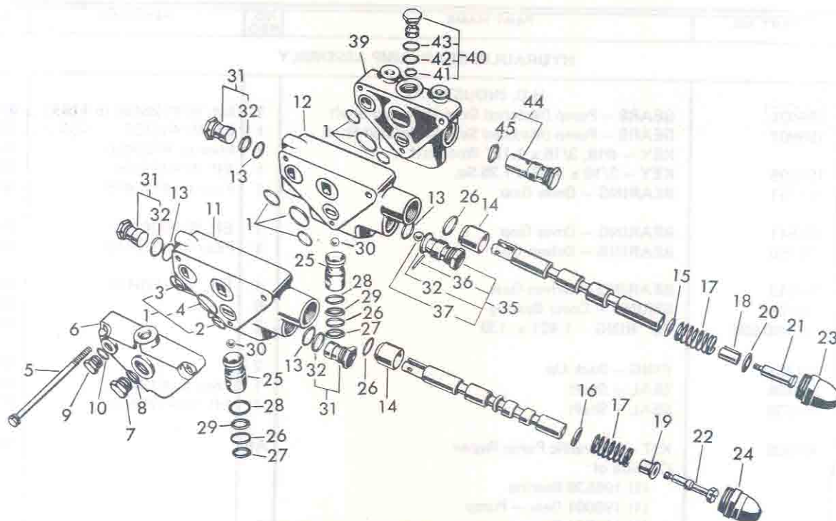
FIG. 5G3 - CONTROL VALVE ASSEMBLY
