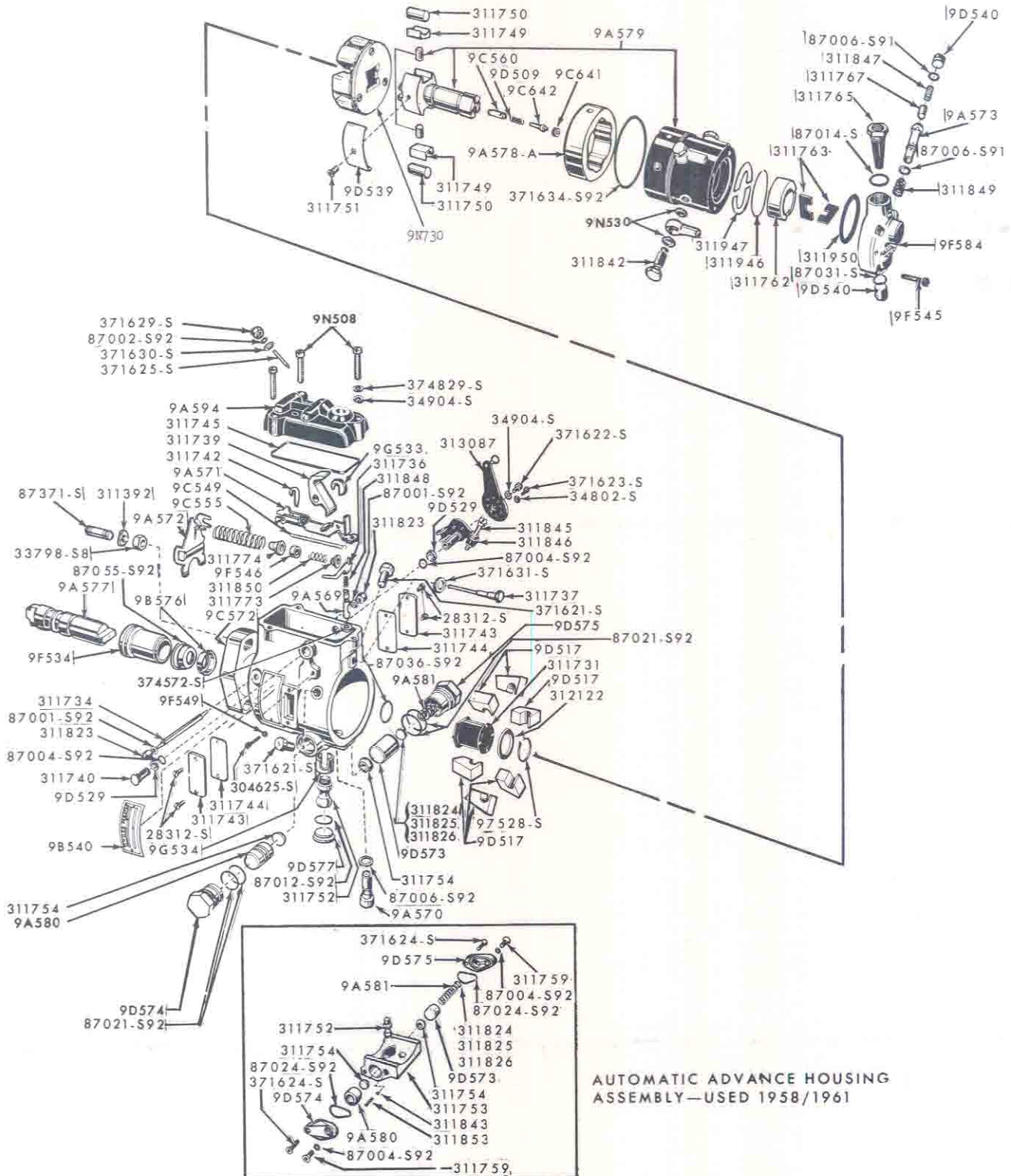
FIG. 9F1 - DIESEL FUEL INJECTION PUMP
