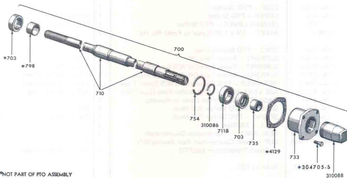
FIG. 7E3 - 1 3/8" P.T.O. ASSEMBLY & RELATED PARTS 1957/
