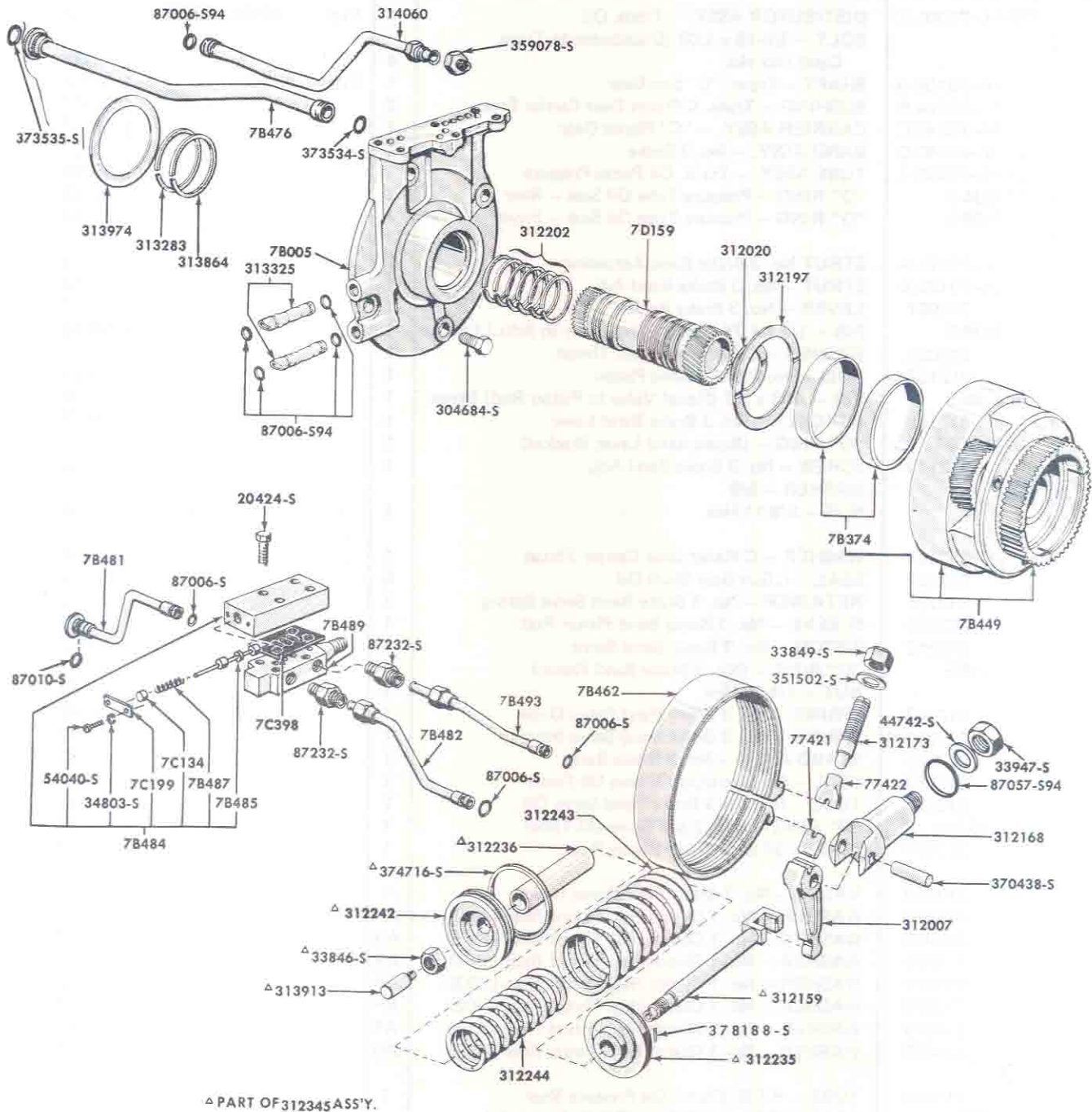
FIG. 7D5 - DISTRIBUTOR, C CARRIER, NO. 3 BRAKE BAND, DIRECT DRIVE CLUTCH VALVE & RELATED PARTS 63/-
