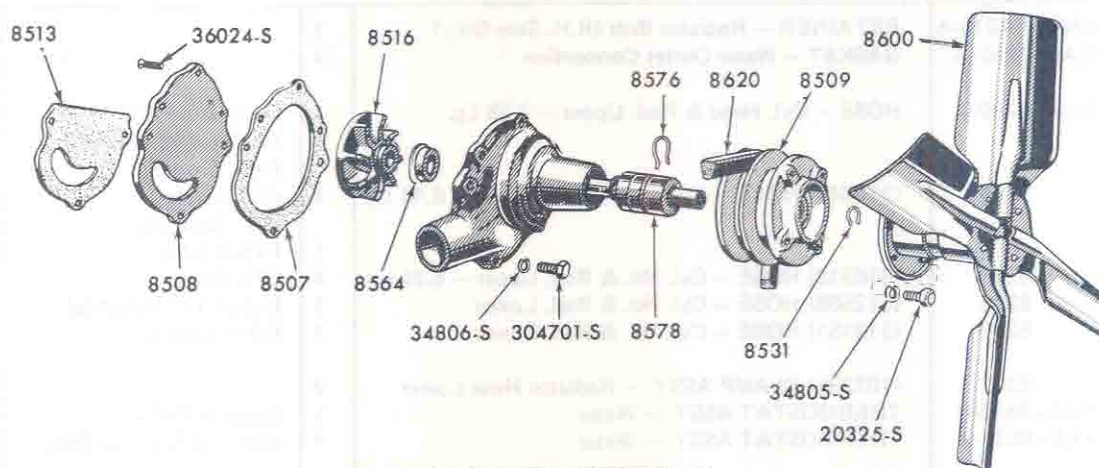
FIG. 8B1 WATER PUMP & RELATED PARTS "NAA" 1953/54
