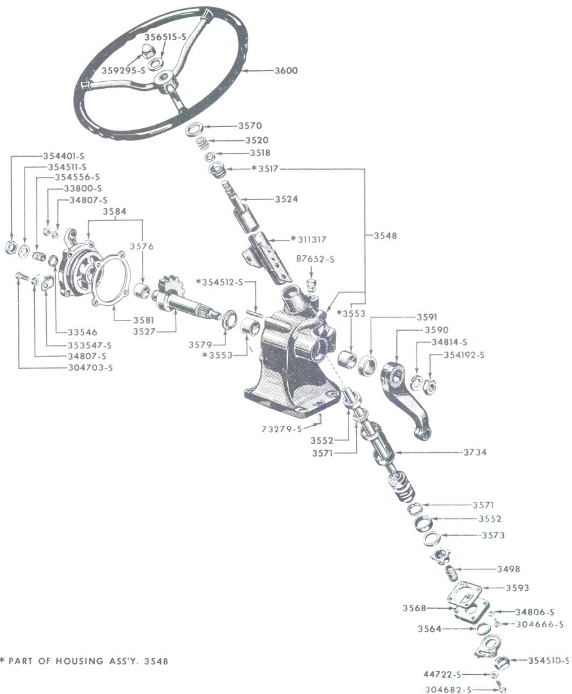
FIG. 3B3 - ROWCROP STEERING GEAR & RELATED PARTS
