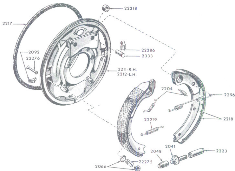
FIG. 2A2 - BRAKES & RELATED PARTS 1955/
