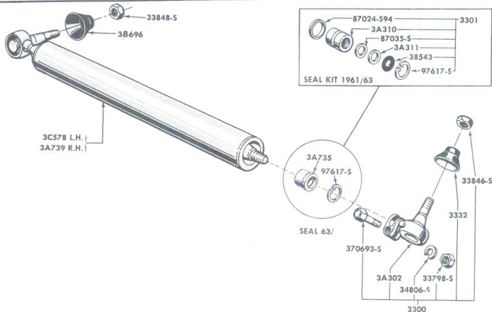
FIG. 3D3 - POWER STEERING CYLINDER ASSEMBLY & RELATED PARTS
