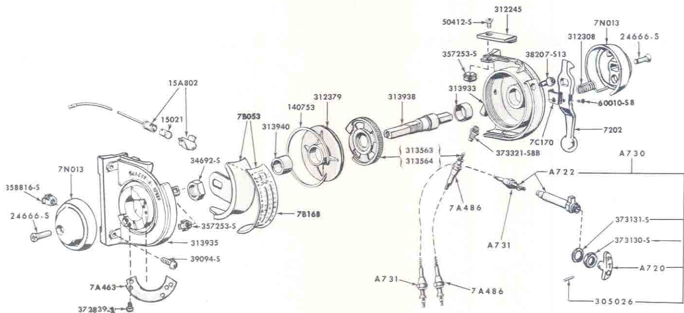
FIG. 7D12 — CONTROL SELECTOR ASSEMBLY &amp; RELATED PARTS 59/-
