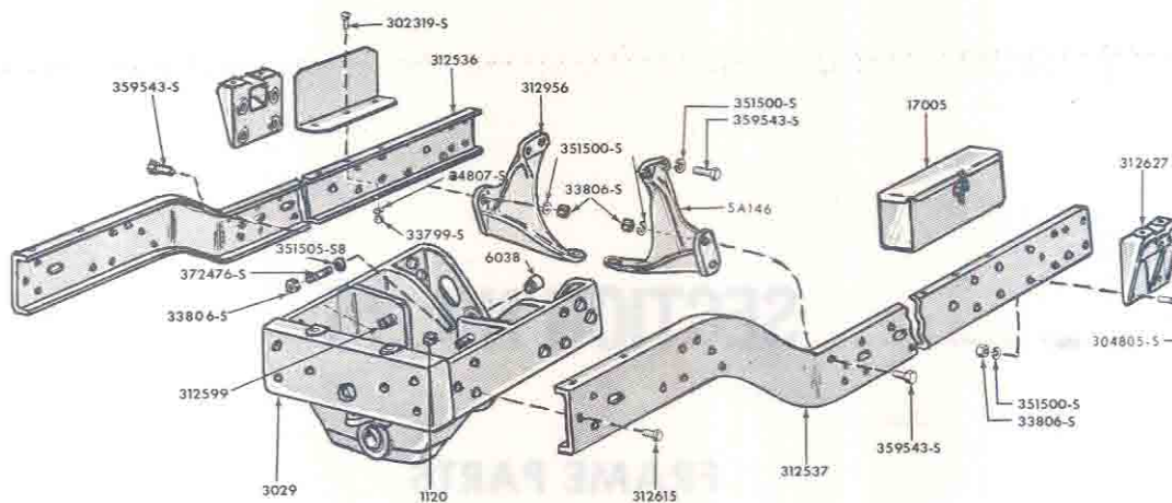
FIG. 15A1 - FRAME & RELATED PARTS
