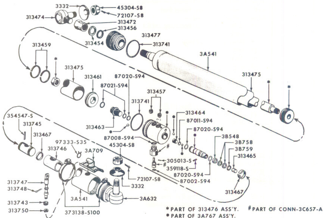
FIG. 3D4 - POWER STEERING CYLINDER & RELATED PARTS 1958/
