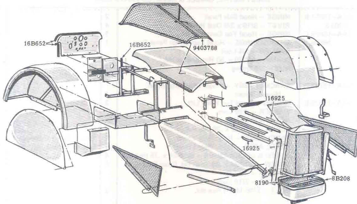
FIG. 14B4 - SHEET METAL, GRILLE & RELATED PARTS
