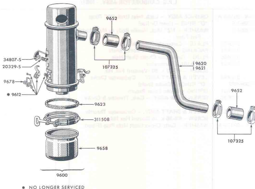
FIG. 9C1 - AIR CLEANER & RELATED PARTS 1953/57
