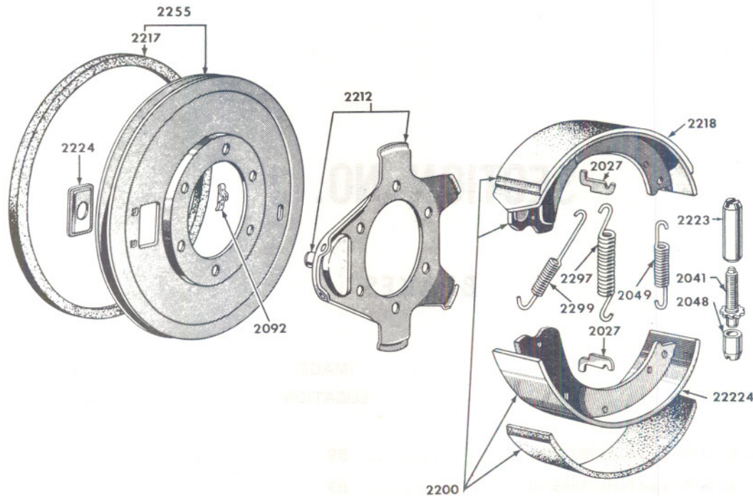
FIG. 2A1 - BRAKES & RELATED PARTS 1953/54
