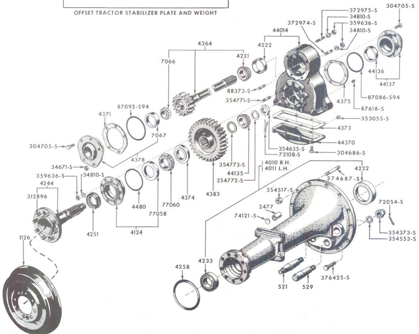
FIG. 4A3 - REAR AXLE SHAFT, HOUSING, FINAL DRIVE & RELATED PARTS
