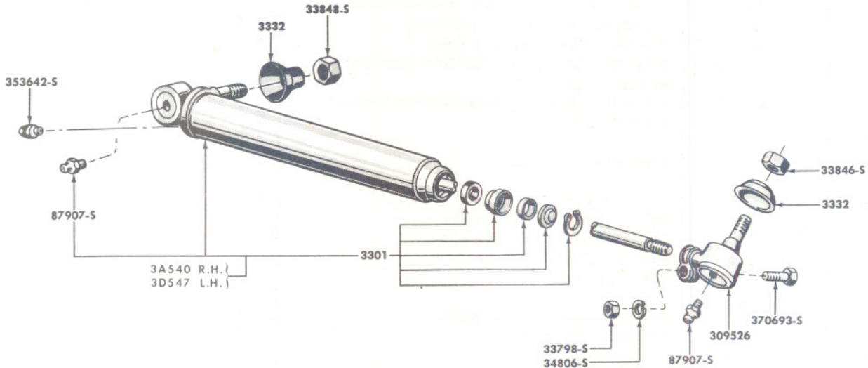
FIG. 3D2 - POWER STEERING CYLINDER ASSEMBLY & RELATED PARTS
