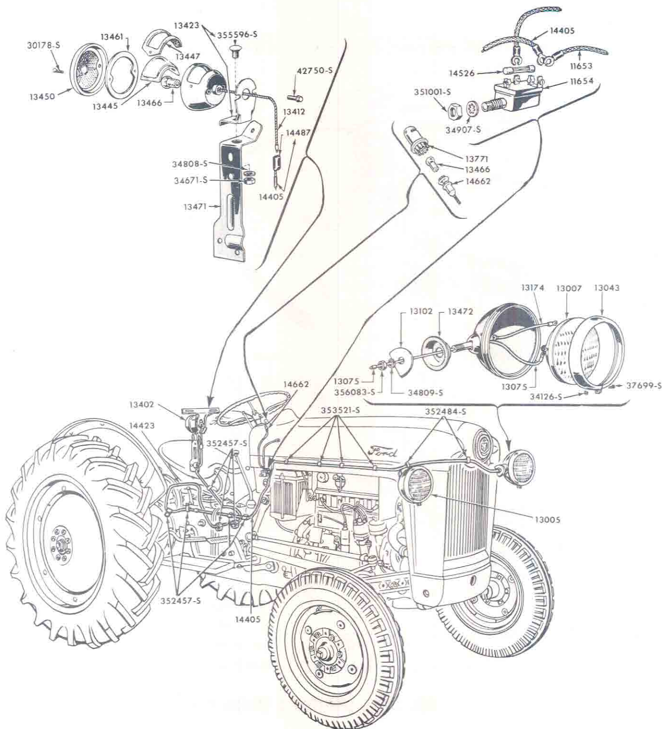
FIG. 11A2 - LIGHTING & WIRING 1953/54
