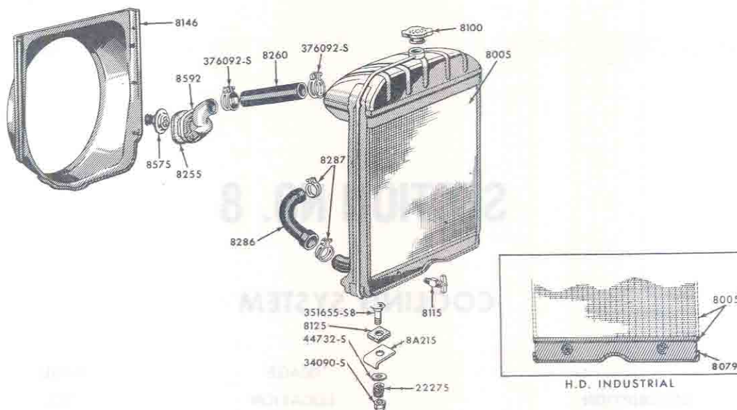
FIG 8A1 - RADIATOR & RELATED PARTS
