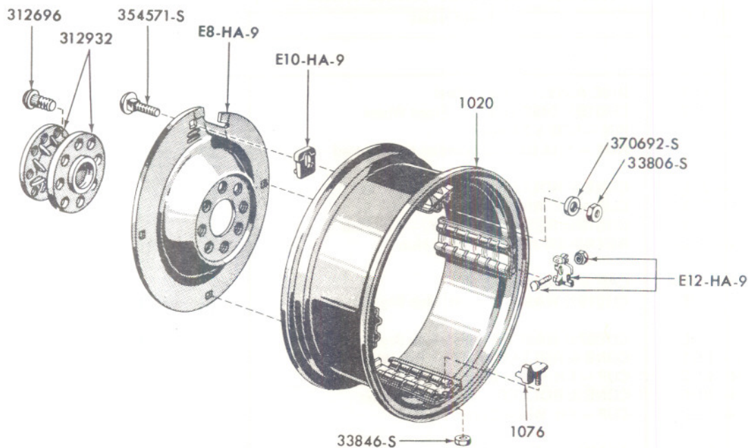
FIG. 1B2 - POWER ADJUSTABLE REAR WHEELS
