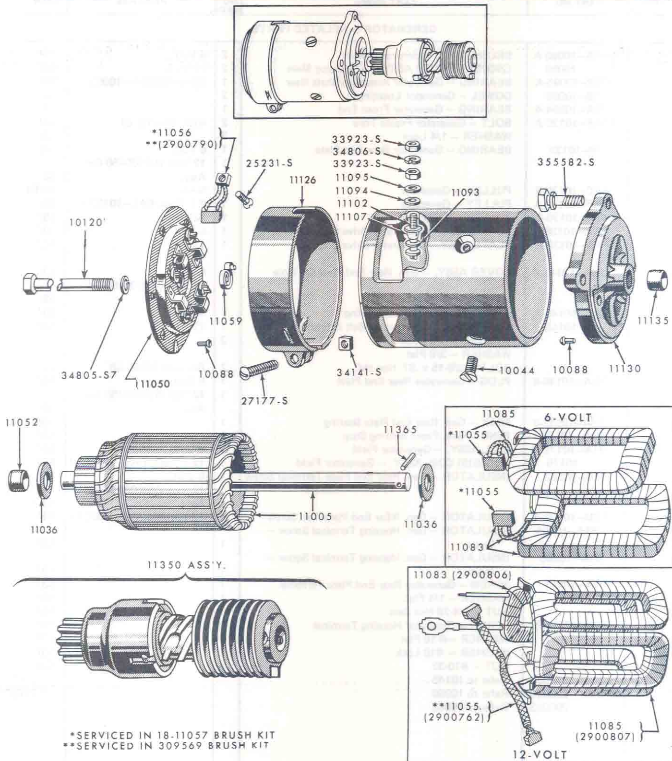
FIG. 11C - STARTER MOTOR & RELATED PARTS
