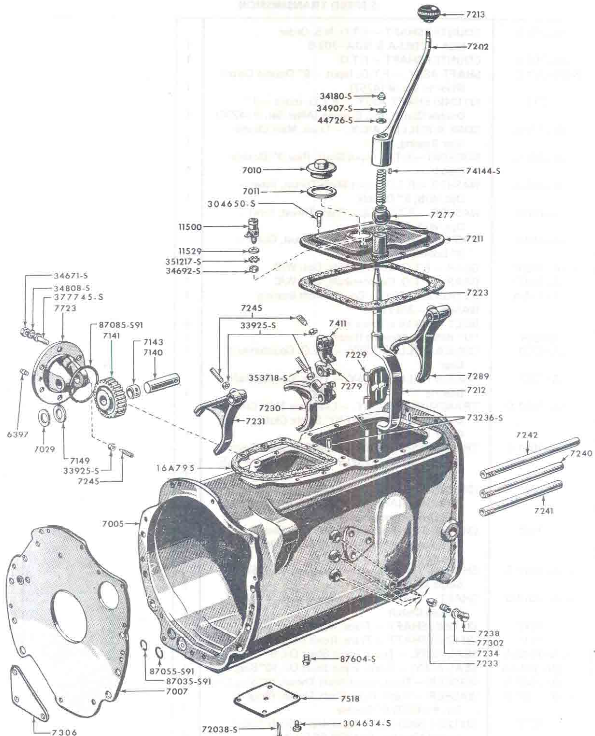
FIG. 7B2 - 5 SPEED TRANS. CASE & RELATED PARTS
