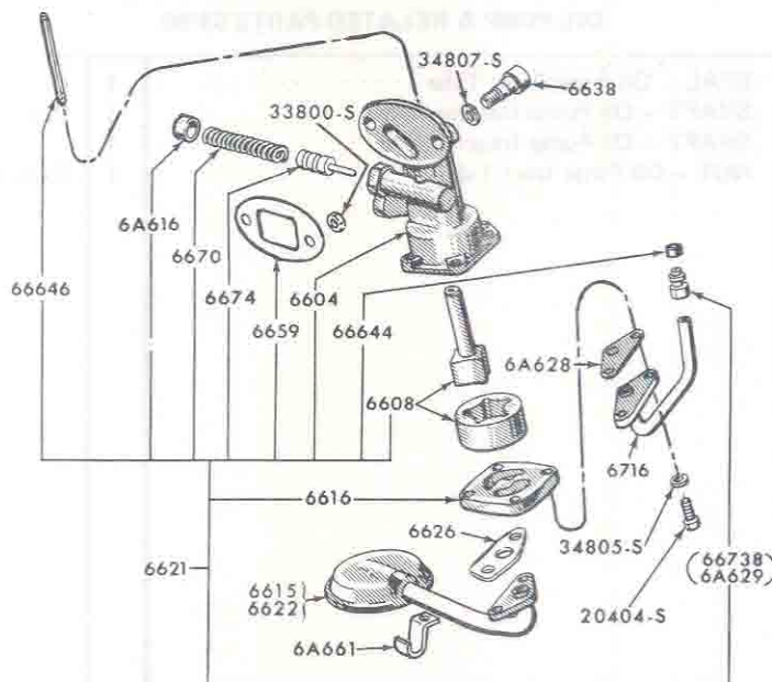
FIG. 6C2 OIL PUMP & RELATED PARTS 61/
