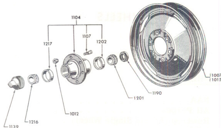
FIG. 1A1 - FRONT WHEEL ASSEMBLY
