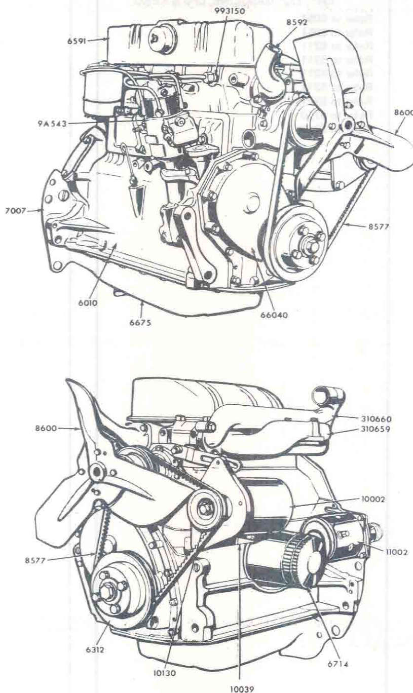
FIG. 6B1- DIESEL ENGINE ASSY. COMPLETE 1958/
