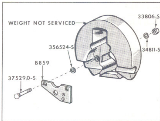
OFFSET TRACTOR STABILIZER PLATE AND WEIGHT
