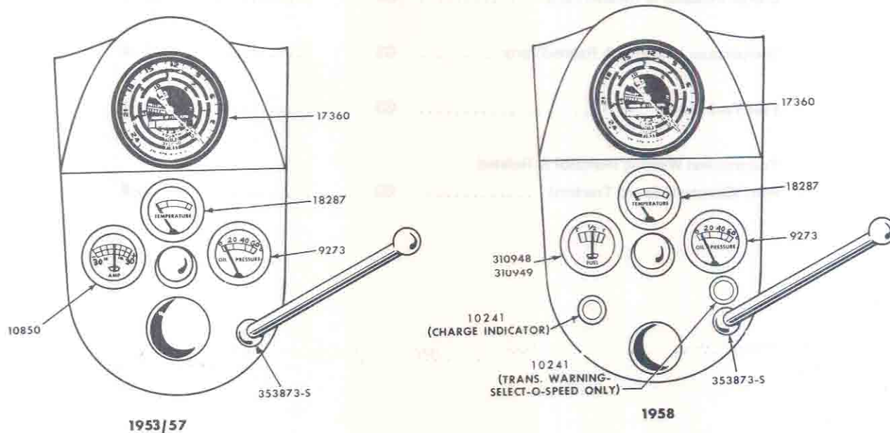
FIG. 12B1 - INSTRUMENT PANEL ASSY.
