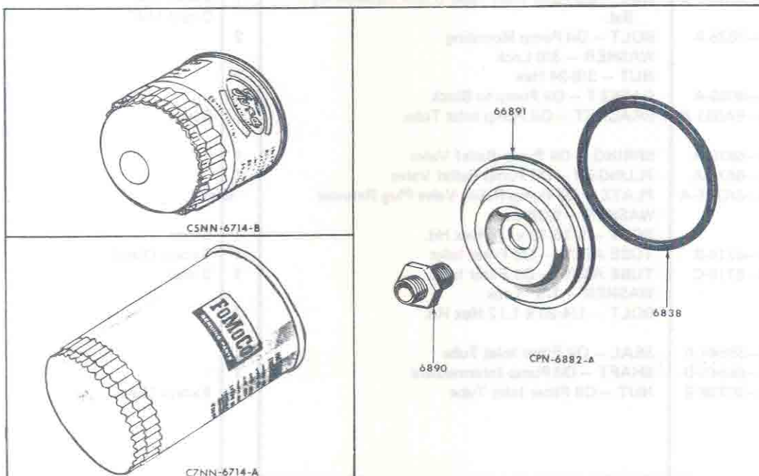
FIG. 6D2 - THROW-AWAY OIL FILTER & RELATED PARTS
