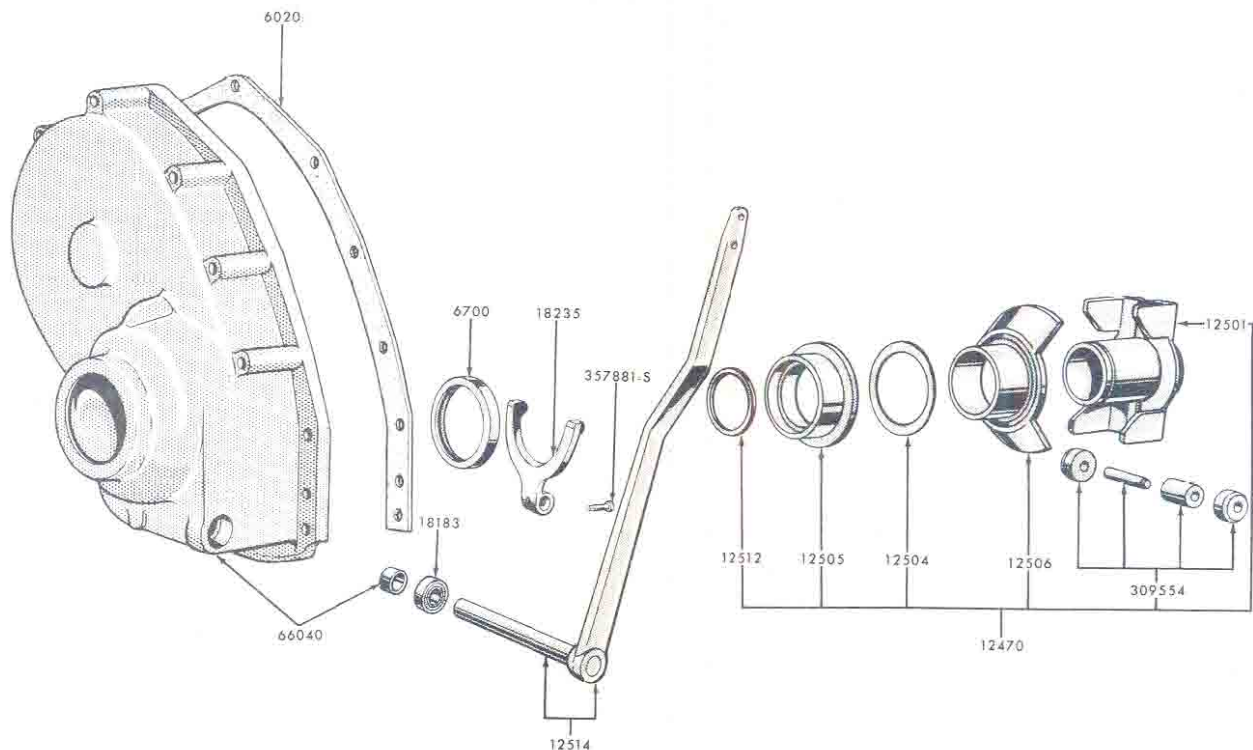
FIG. 6G2 GOVERNOR ASSY. - 1958/ - AFTER SER. #26402
