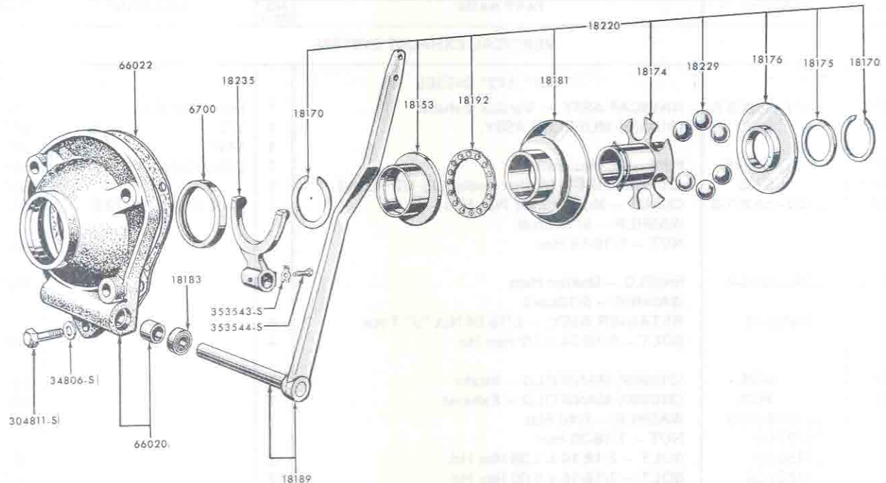
FIG. 6G1 GOVERNOR ASSY. - 1953/58 - PRIOR TO SER. #26403
