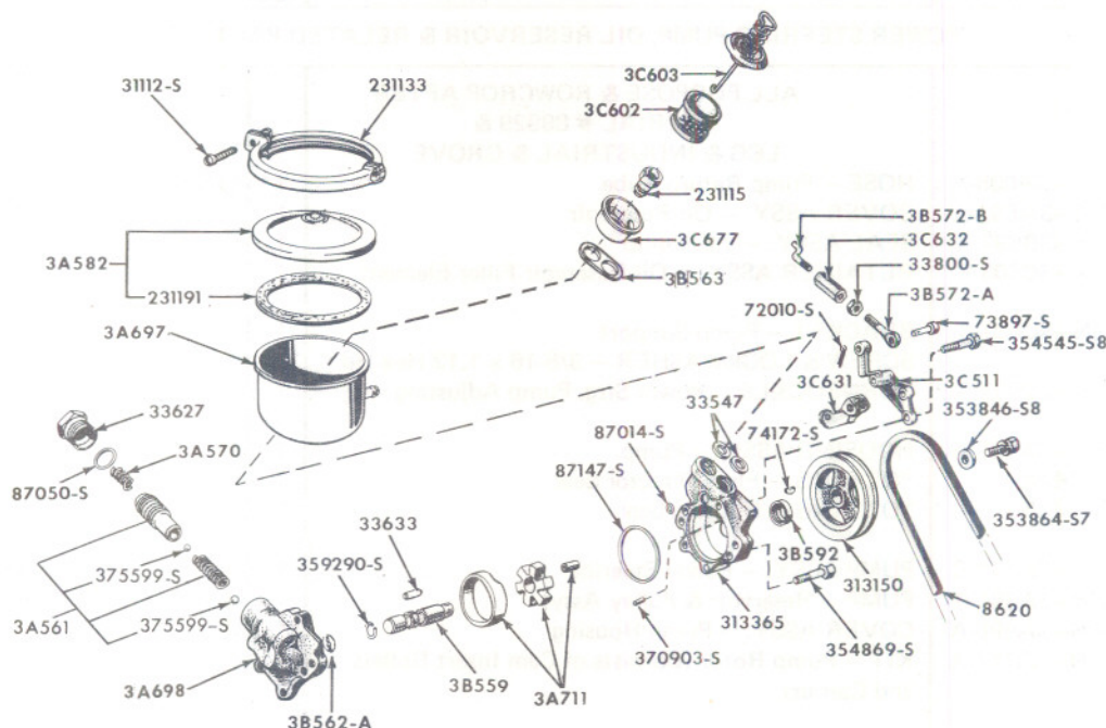
FIG. 3C4 - POWER STEERING PUMP, OIL RESERVOIR & RELATED PARTS
