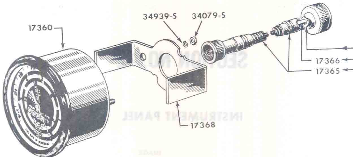
FIG. 12A1 - PROOFMETER & RELATED PARTS
