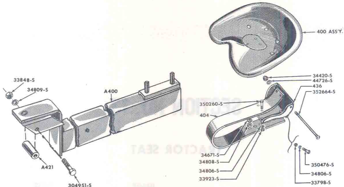
FIG. 13A1 - STANDARD SEAT & RELATED PARTS
