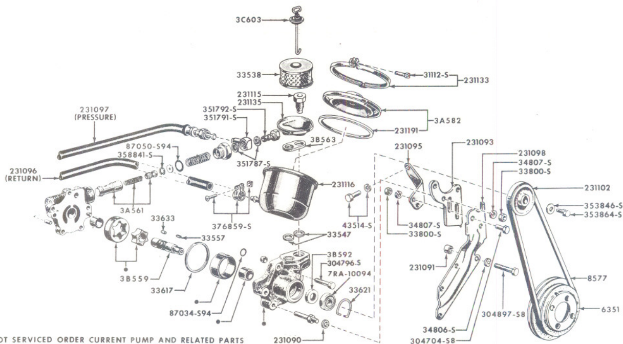
FIG. 3C1 - POWER STEERING PUMP, OIL RESERVOIR & RELATED PARTS
