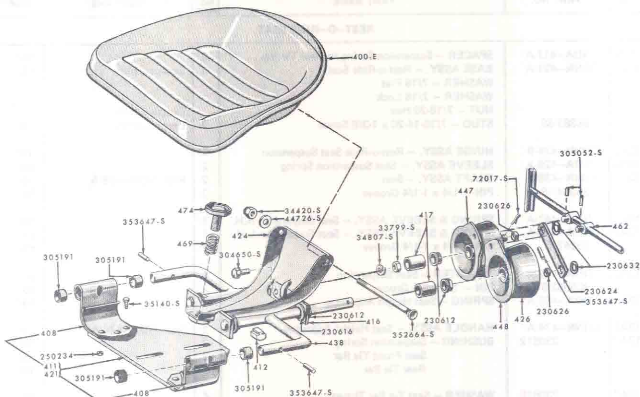
FIG. 13A2 - REST-O-RIDE SEAT
