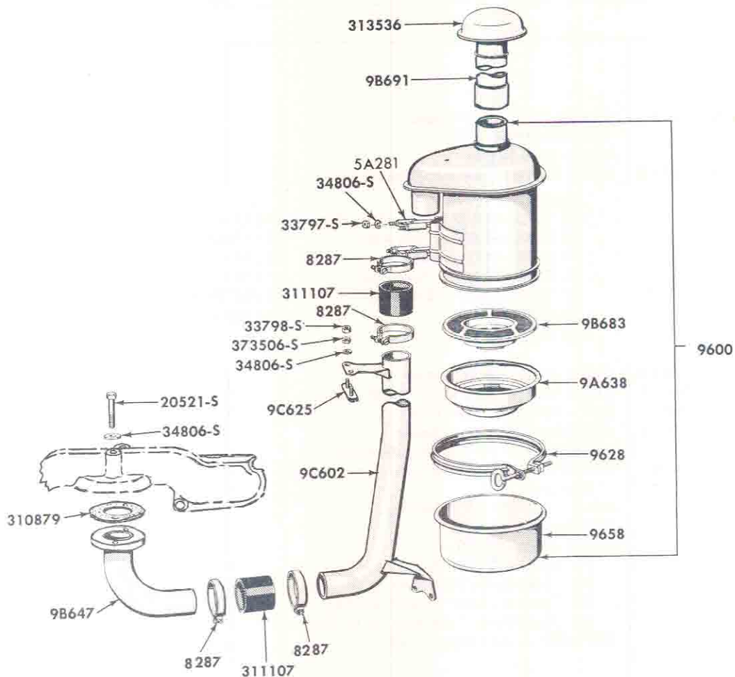
FIG. 9C4 - DIESEL AIR CLEANER & RELATED PARTS, 1963/
