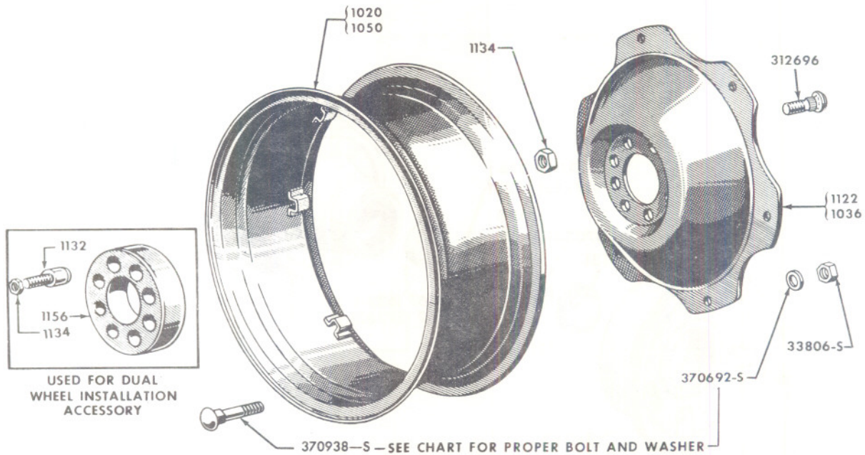
FIG. 1B1 - STANDARD REAR WHEELS
