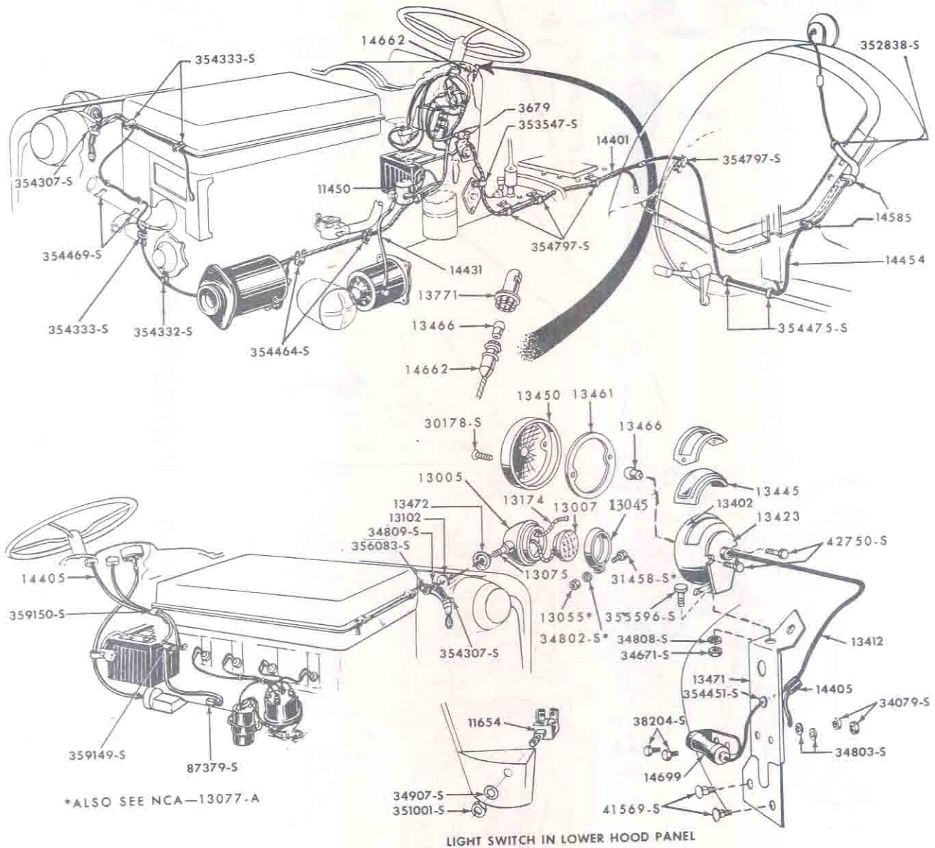
FIG. 11A3 - LIGHTING & WIRING 1955/57
