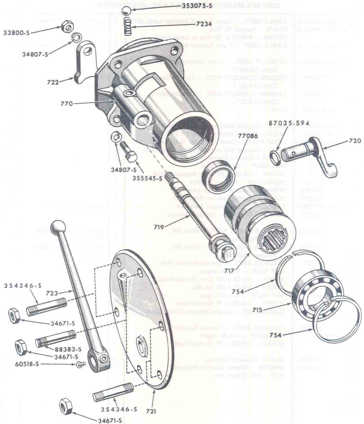
FIG. 7E1 - P.T.O. SUPPORT, SHIFTER LEVER & RELATED PARTS
