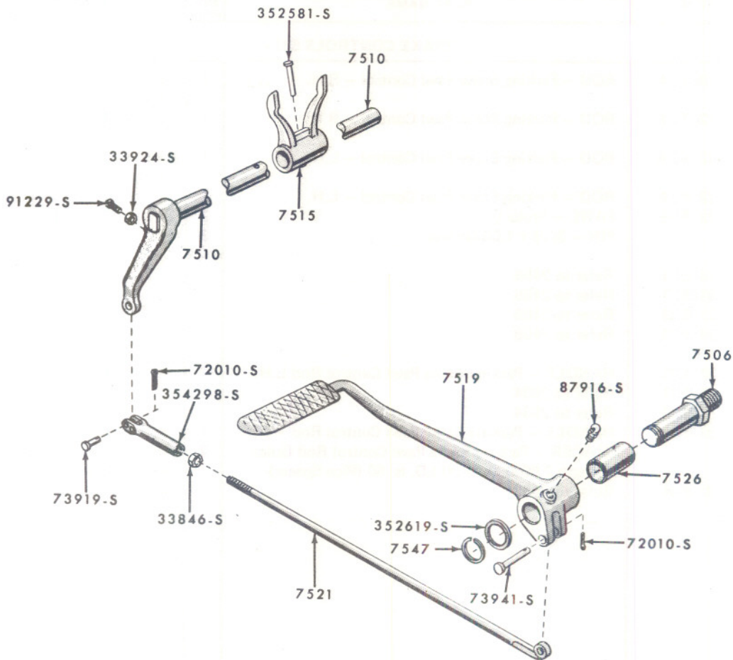
FIG. 2B3 - CLUTCH CONTROLS 58/-
