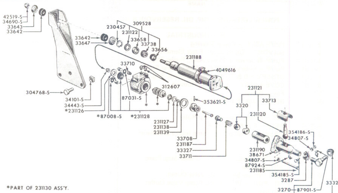
FIG. 3D1 - POWER STEERING CYLINDER ASSEMBLY & RELATED PARTS
