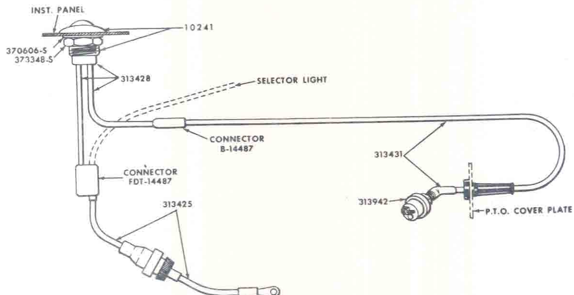
FIG. 12C1 - TRANSMISSION WARNING INDICATOR & RELATED PARTS
