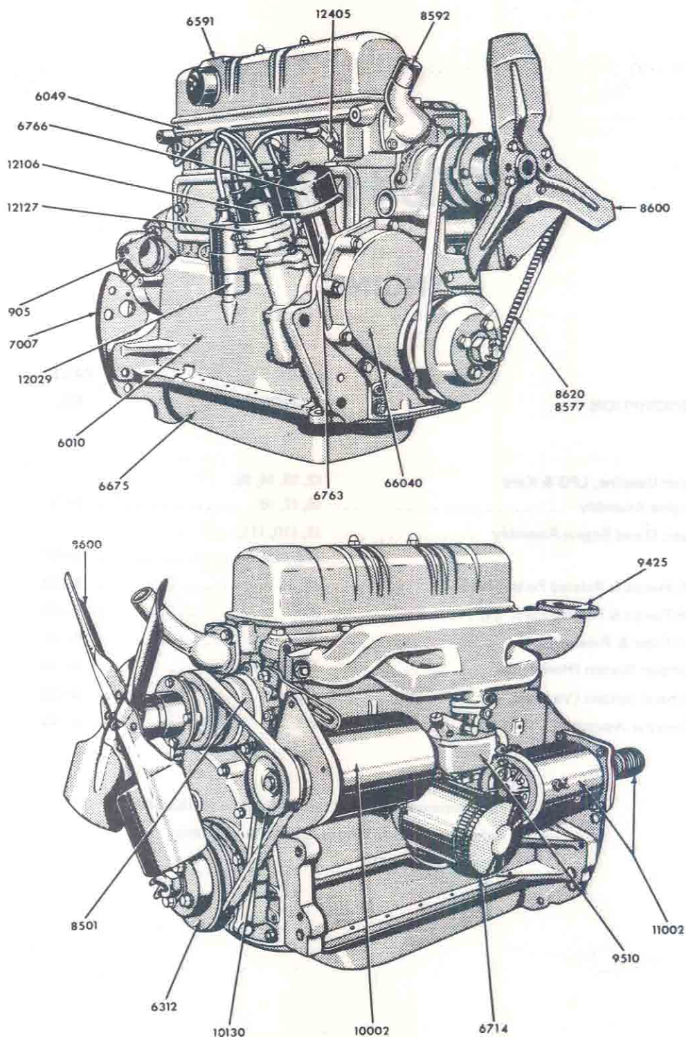
FIG. 6A1 - GASOLINE ENGINE ASSY. COMPLETE 1953/
