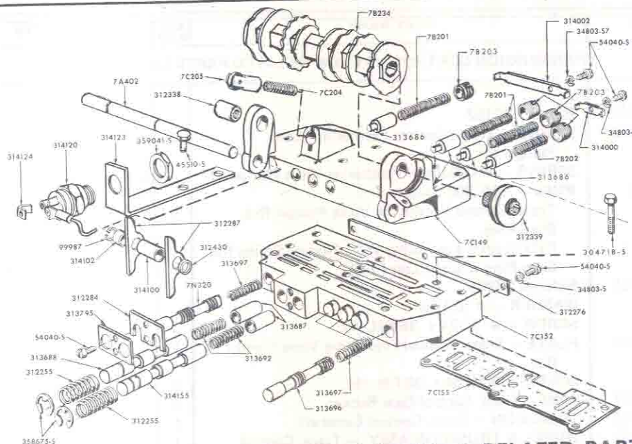
FIG. 7D11 TRANSMISSION CONTROL VALVE & RELATED PARTS 59/
