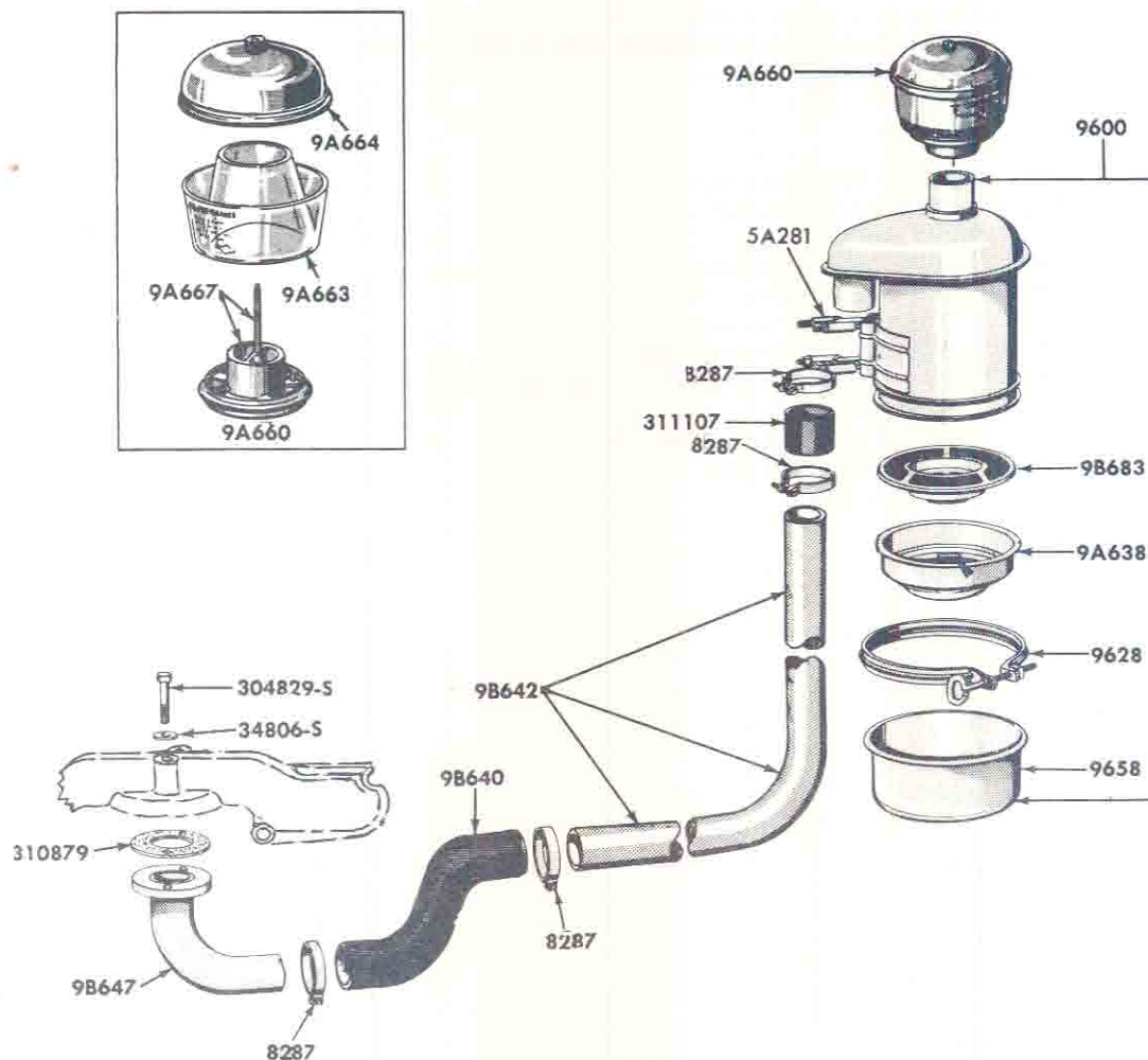
FIG.9C5 - AIR CLEANER & RELATED PARTS 1963/ (GROVE TRACTOR)
