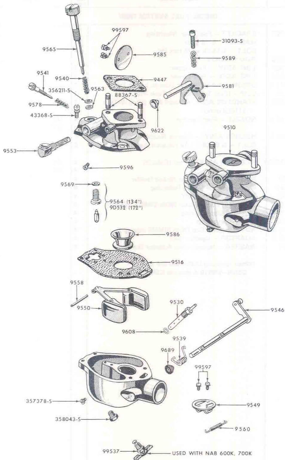
FIG. 9B1 - CARBURETOR ASSY. - 1953/57
