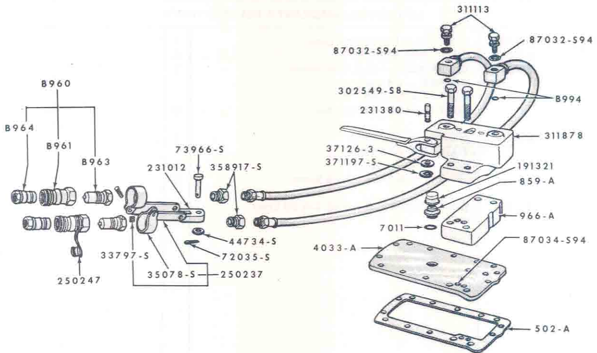
FIG. 5A3A - HYD. VALVE, MANIFOLD & HOSE PARTS (GROVE TRACTOR)
