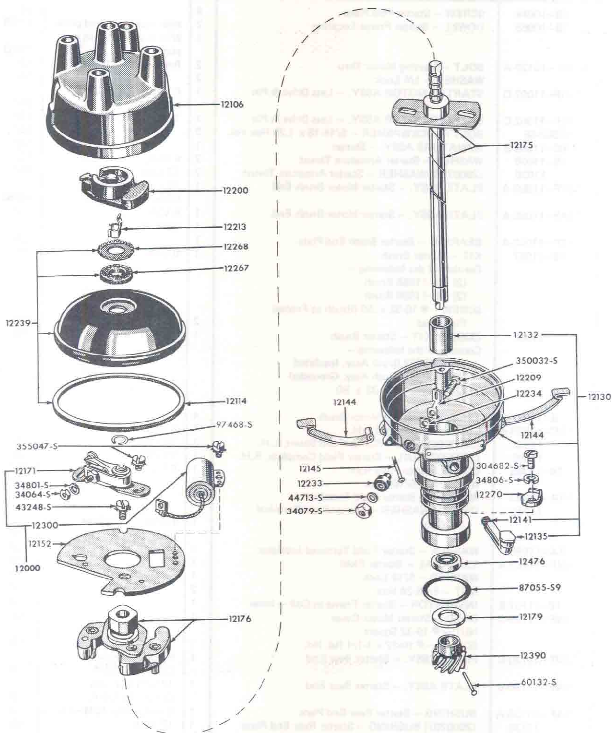
FIG. 11D - DISTRIBUTOR & RELATED PARTS
