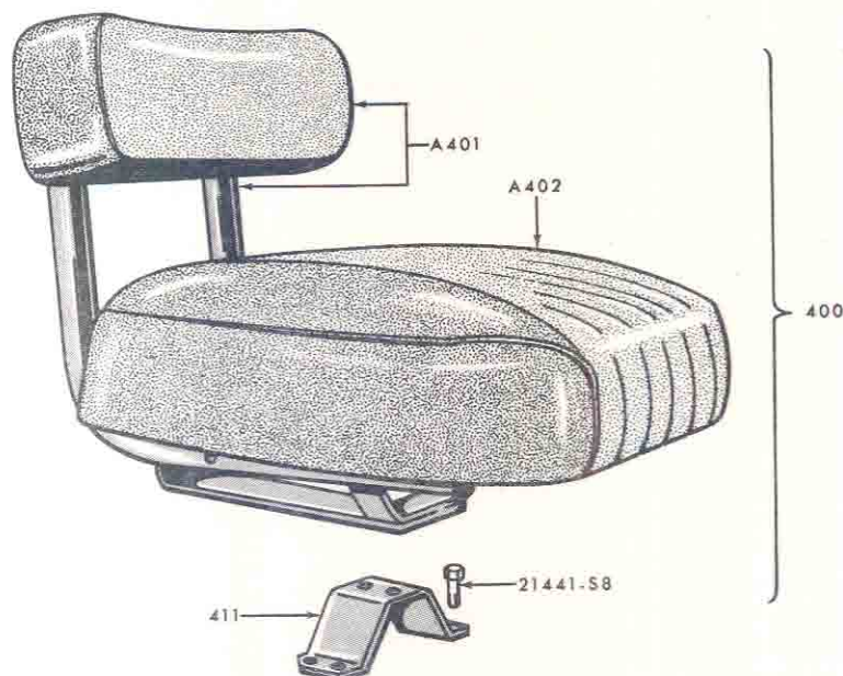
FIG. 13A3 - DELUXE SEAT
