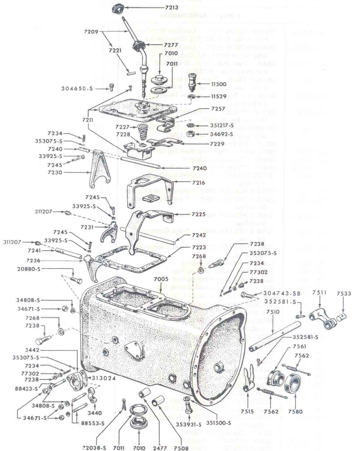
FIG. 7A2 - 4 SPEED TRANS. CASE & RELATED PARTS
