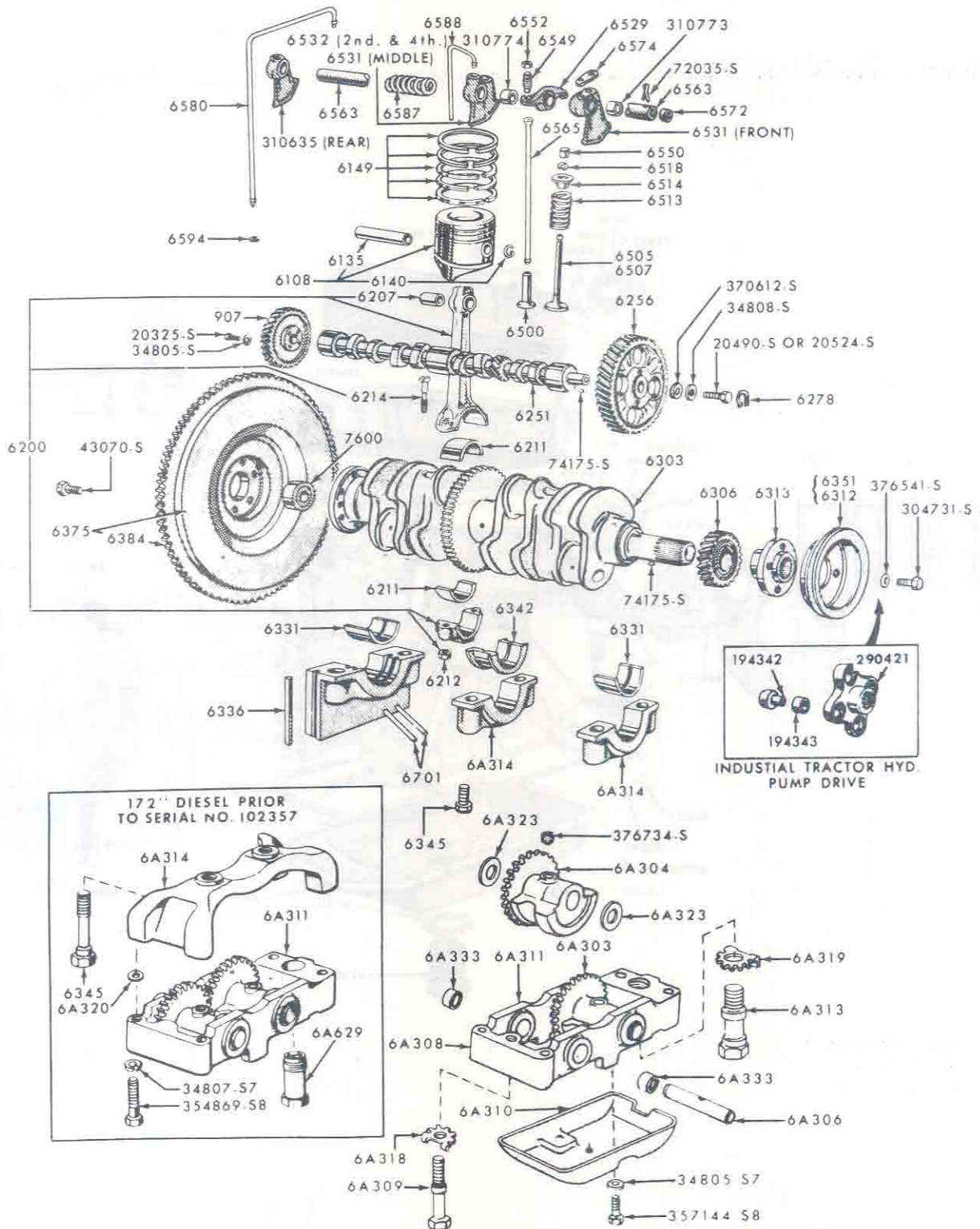
FIG. 6B3 - DIESEL ENGINE ASSY. - INSIDE
