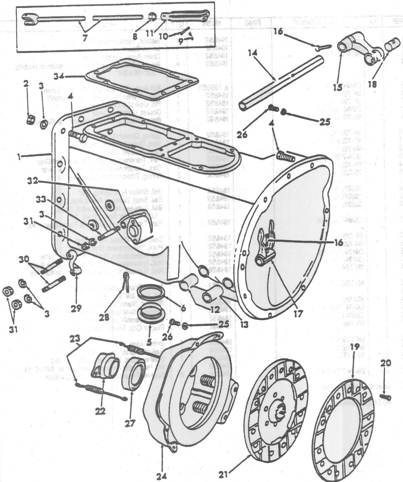
FIG. 7C1 - TRANSMISSION CASE, CLUTCH &amp; RELATED PARTS - 9N, 2N, 8N
