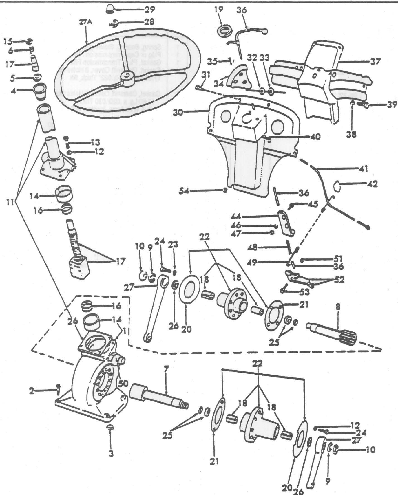
FIG. 3C1 - STEERING GEAR &amp; RELATED PARTS - 8N (BSN 216989)
