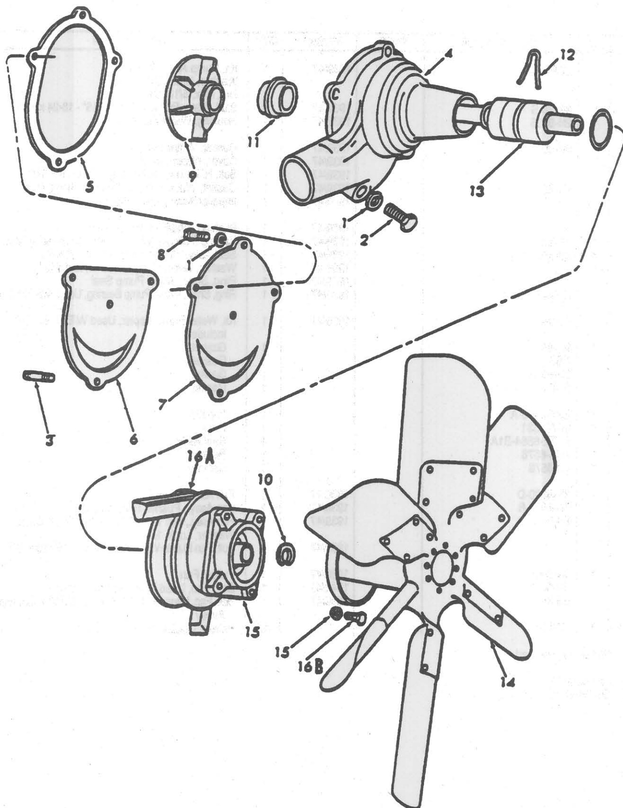
FIG. 8B2 - WATER PUMP ASSY. & RELATED PARTS (1948/52) - 8N
