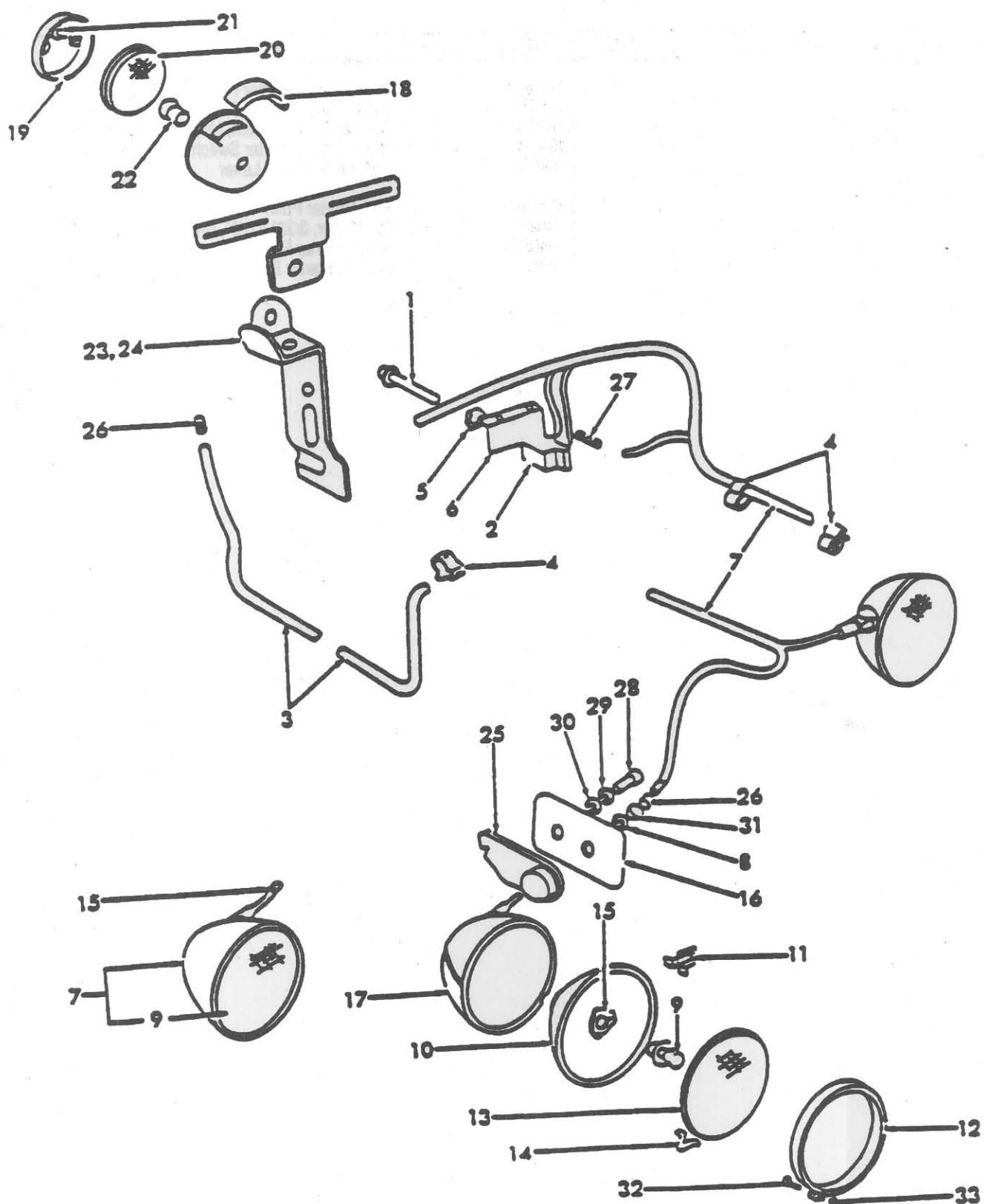
FIG. 11G1 - LIGHTING KIT & WIRING - 9N,2N
