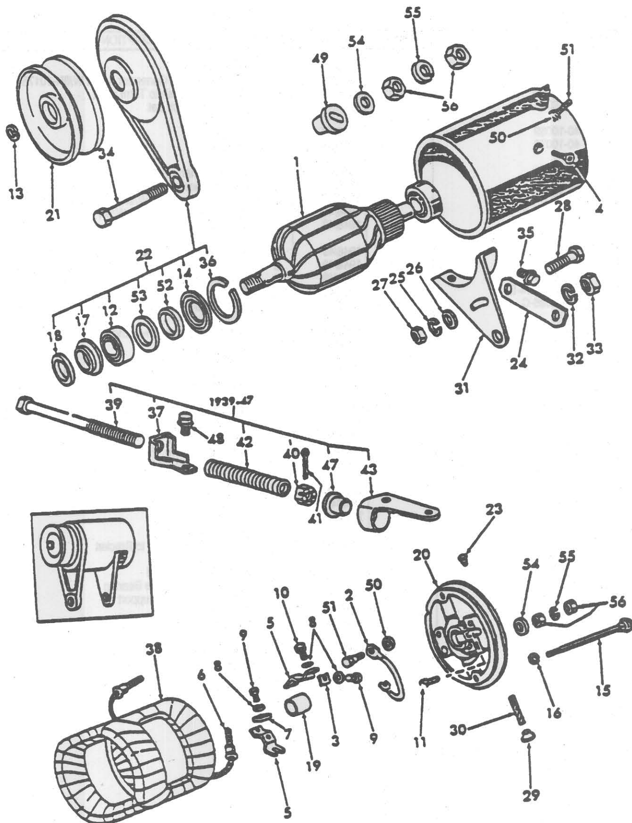
FIG. 11B1 - GENERATOR & RELATED PARTS (3 BRUSH) 8N PRIOR TO S/N 263844 - 1948/49
