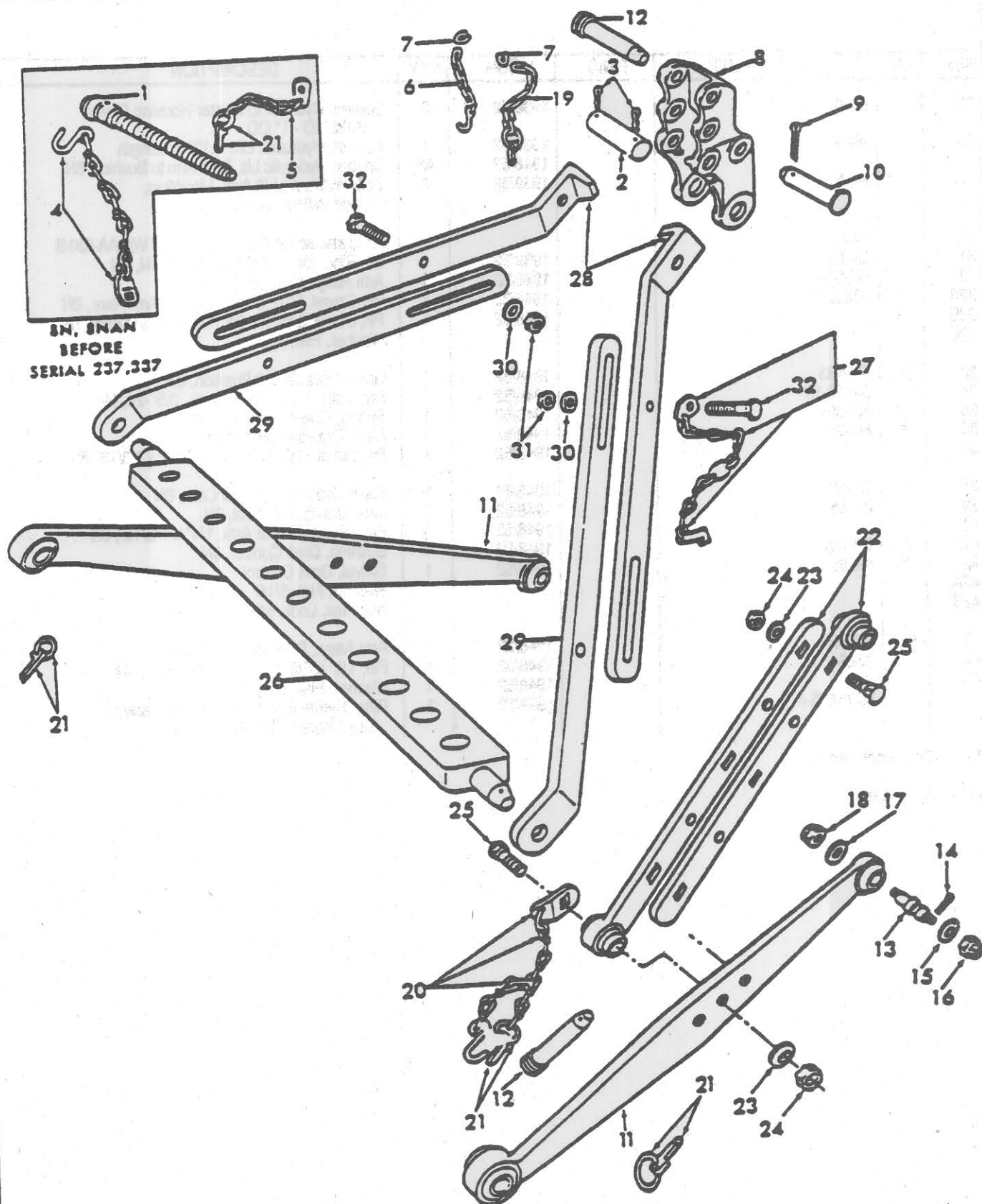
FIG. 5C1 - HYDRAULIC LIFT LINKS &amp; RELATED PARTS - 9N, 2N, 8N
