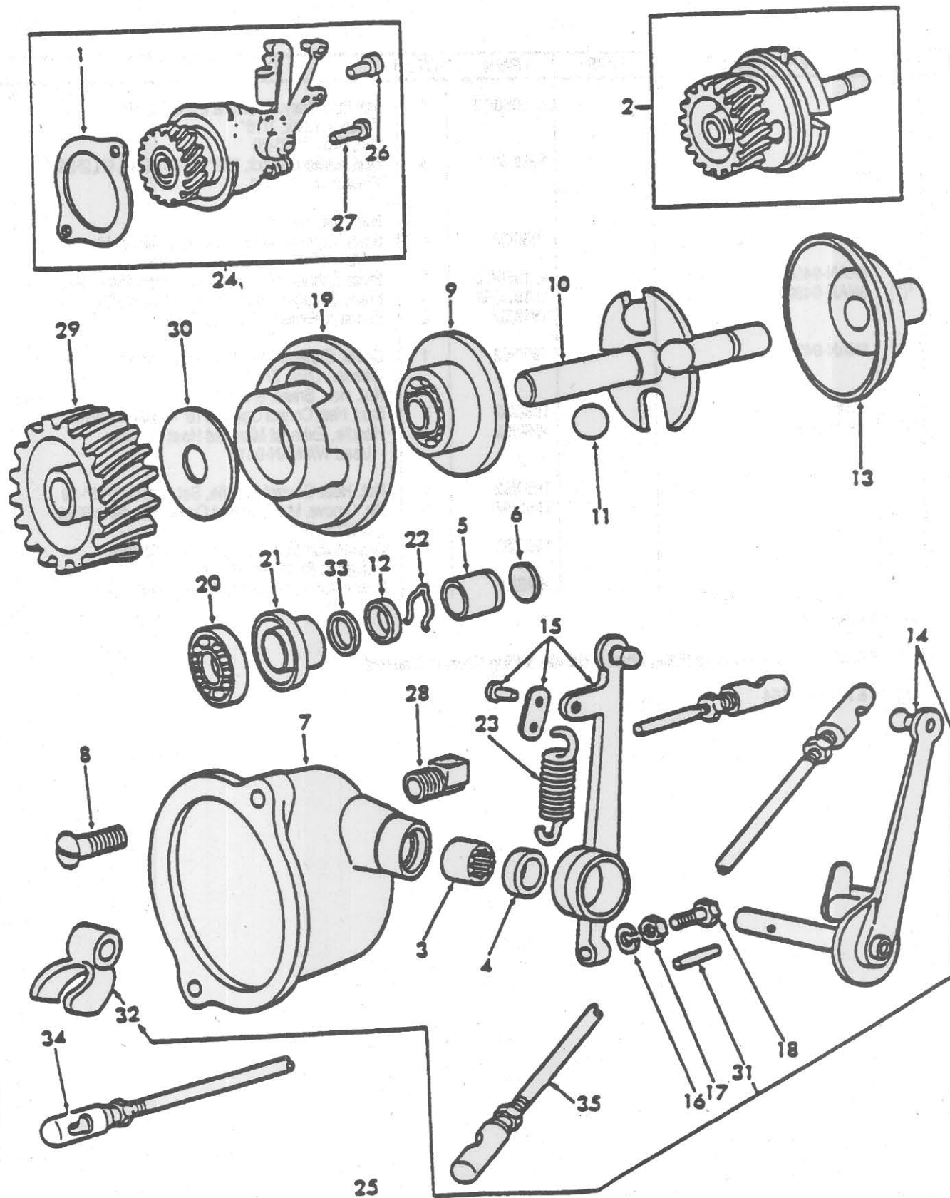
FIG. 6G1 - GOVERNOR &amp; RELATED PARTS - 9N, 2N, 8N
