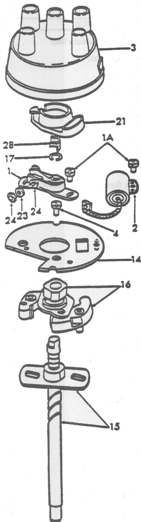
FIG. 11D2 - DISTRIBUTOR - 8N AFTER S/N 263843
