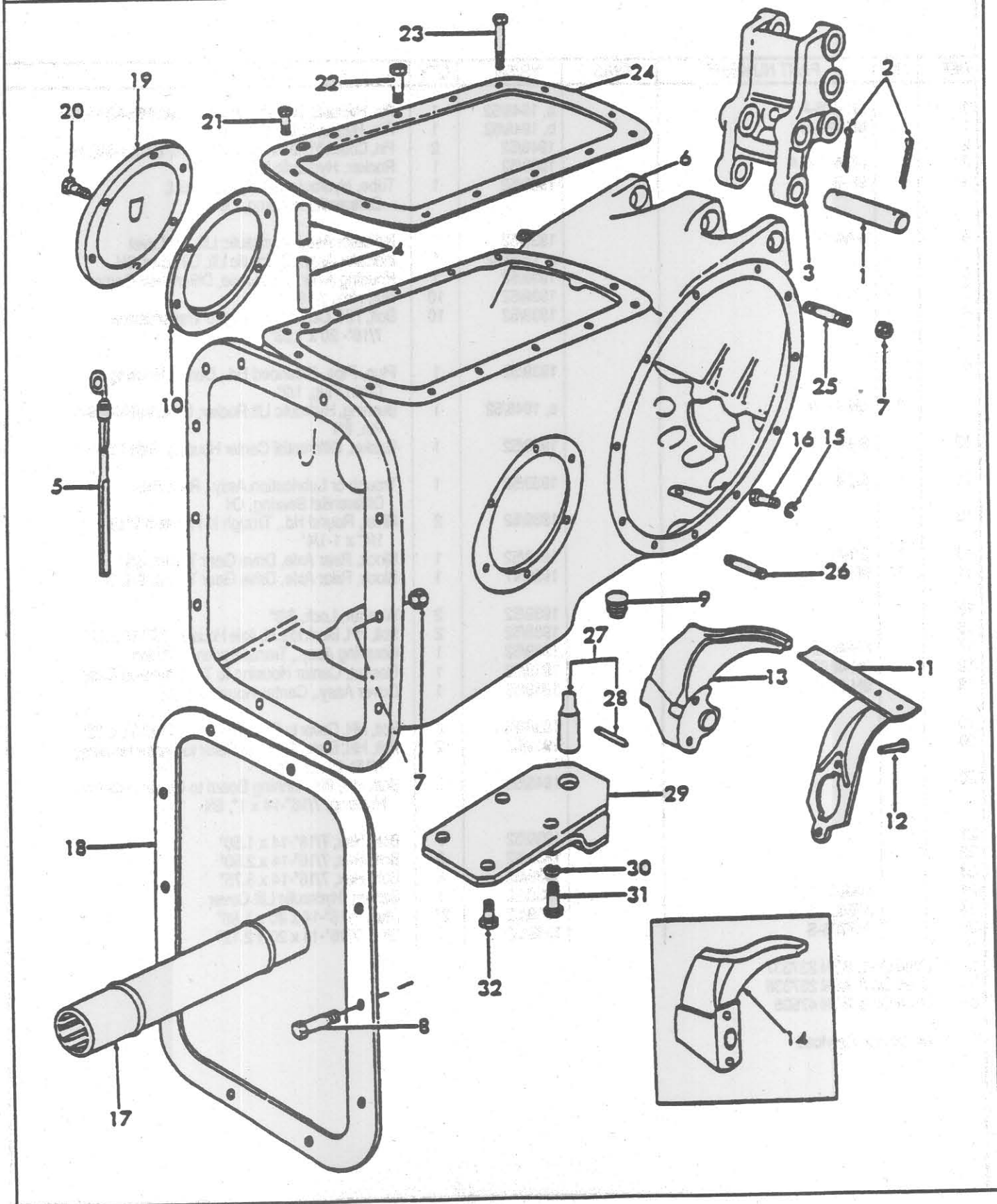
FIG. 4C1 - CENTER HOUSING, ROCKER &amp; RELATED PARTS - 9N, 2N, 8N
