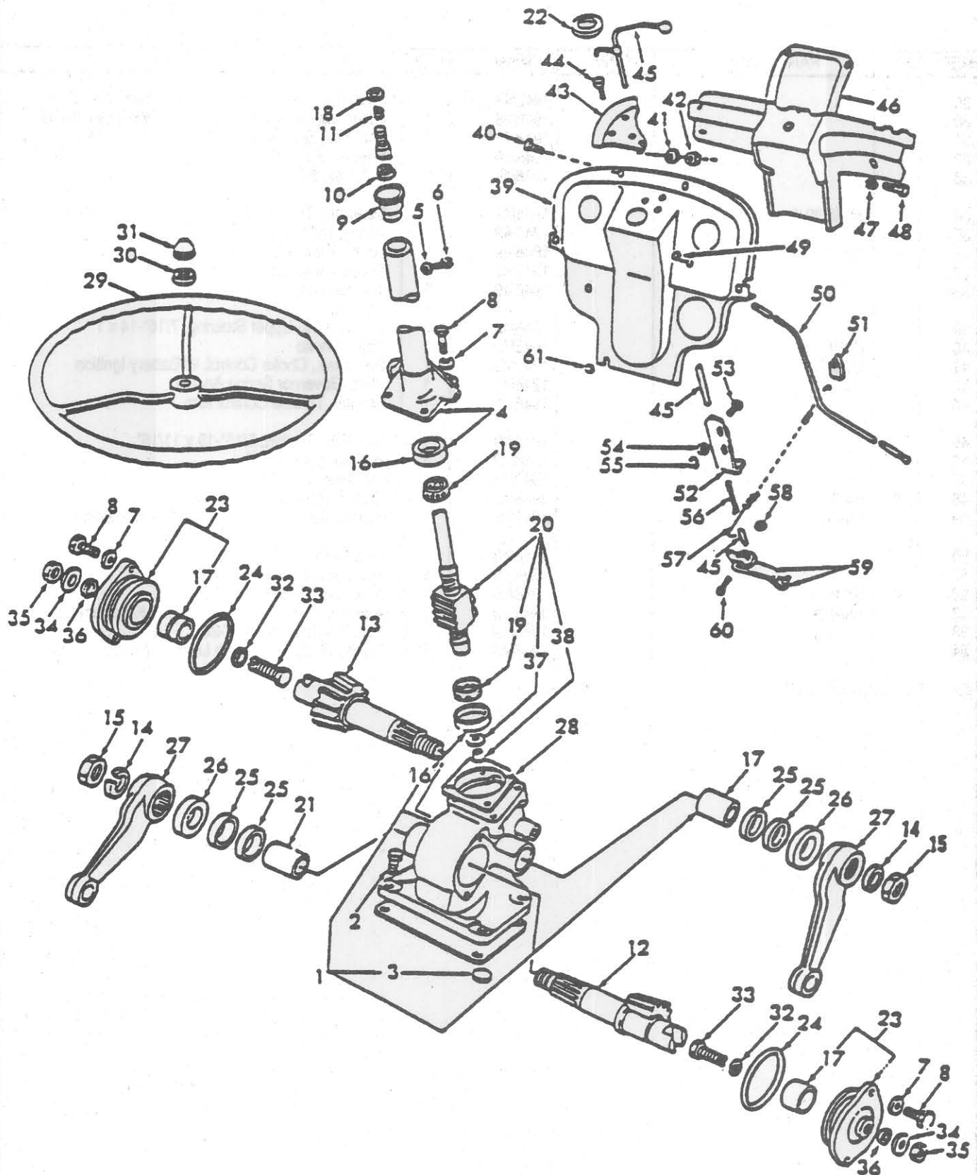
FIG. 3C2 - STEERING GEAR &amp; RELATED PARTS - 8N (ASN 216988)
