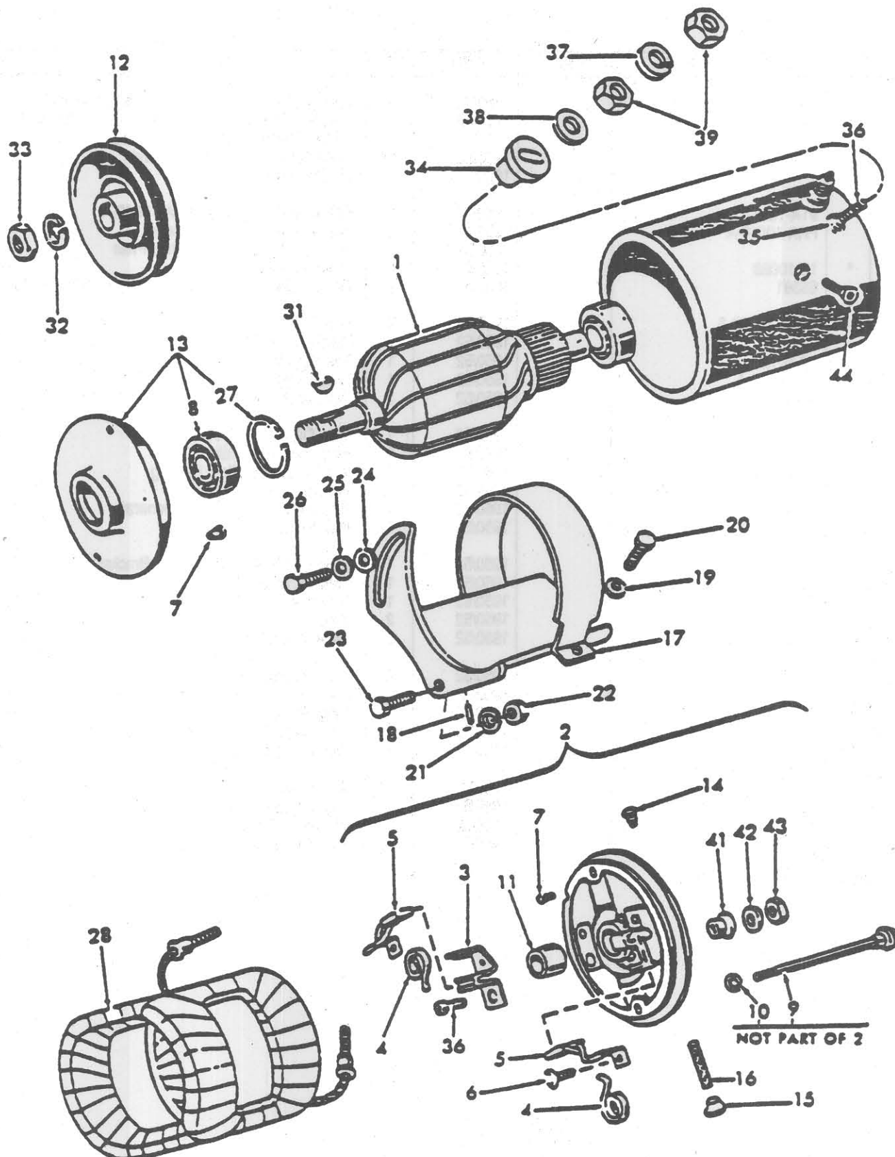
FIG. 11B3 - GENERATOR ASSY. &amp; RELATED PARTS - (2 BRUSH) - 8N AFTER S/N 2638
