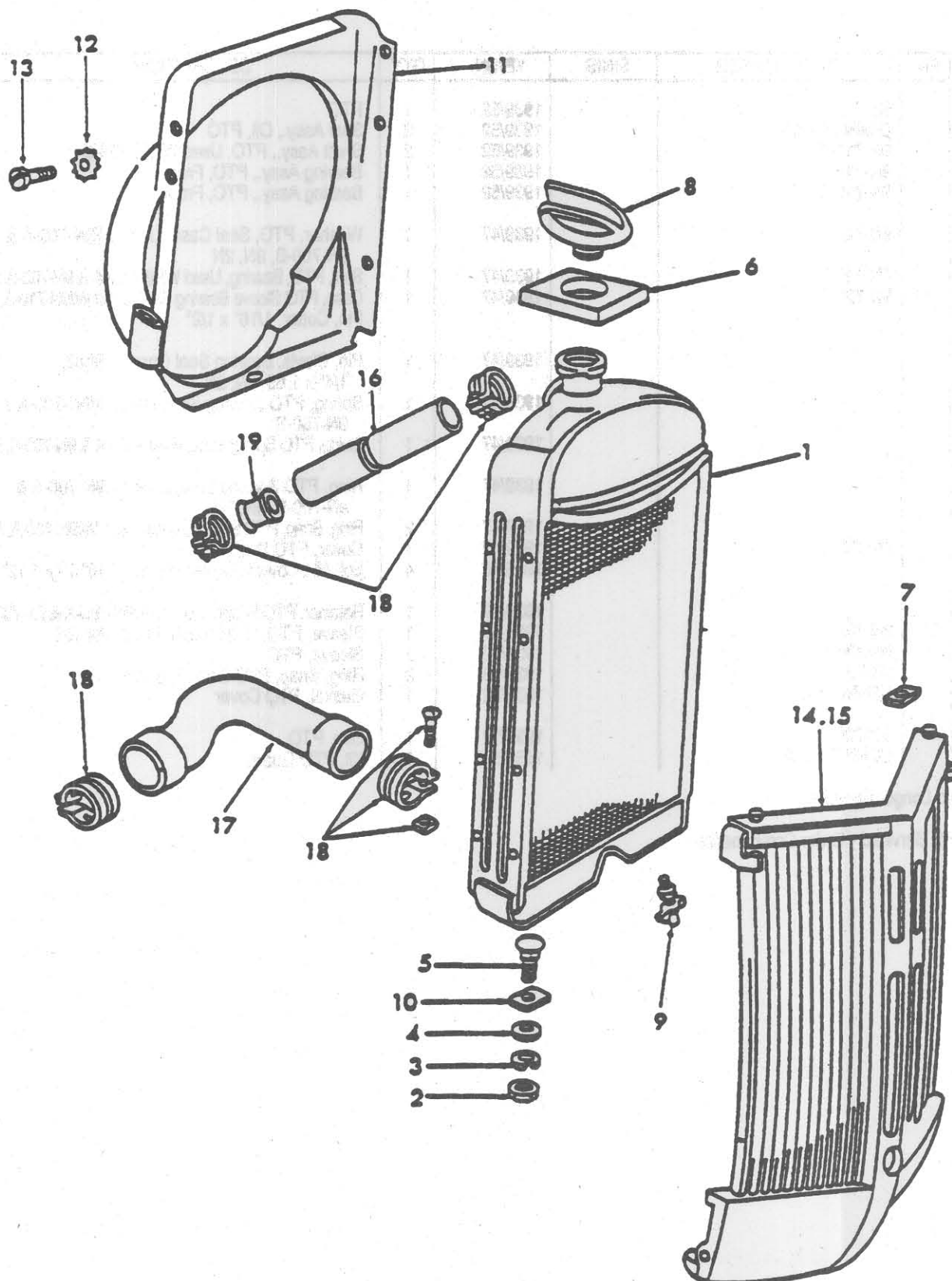
FIG. 8A1 - RADIATOR & RELATED PARTS - 9N, 2N, 8N
