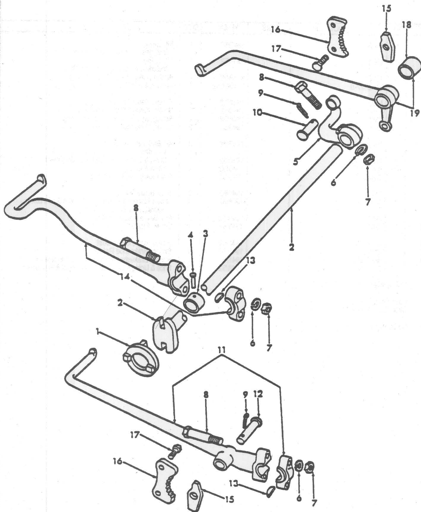
FIG. 2B1 - BRAKE CONTROLS &amp; RELATED PARTS - 9N, 2N
