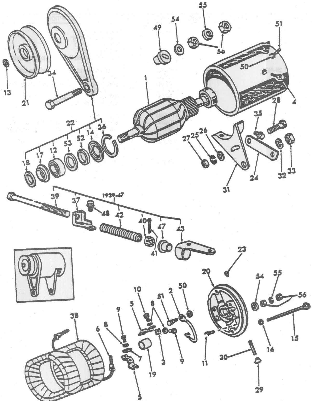
FIG. 11B1 - GENERATOR &amp; RELATED PARTS (3 BRUSH) 8N PRIOR TO S/N 263844 - 1948/49
