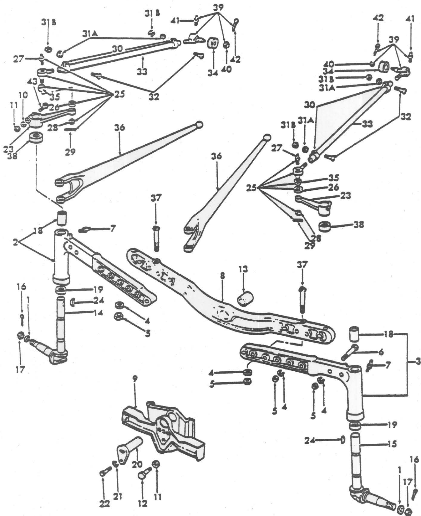
FIG. 3A1 - FRONT AXLE & RELATED PARTS (1939/52) - 9N, 2N, 8N
