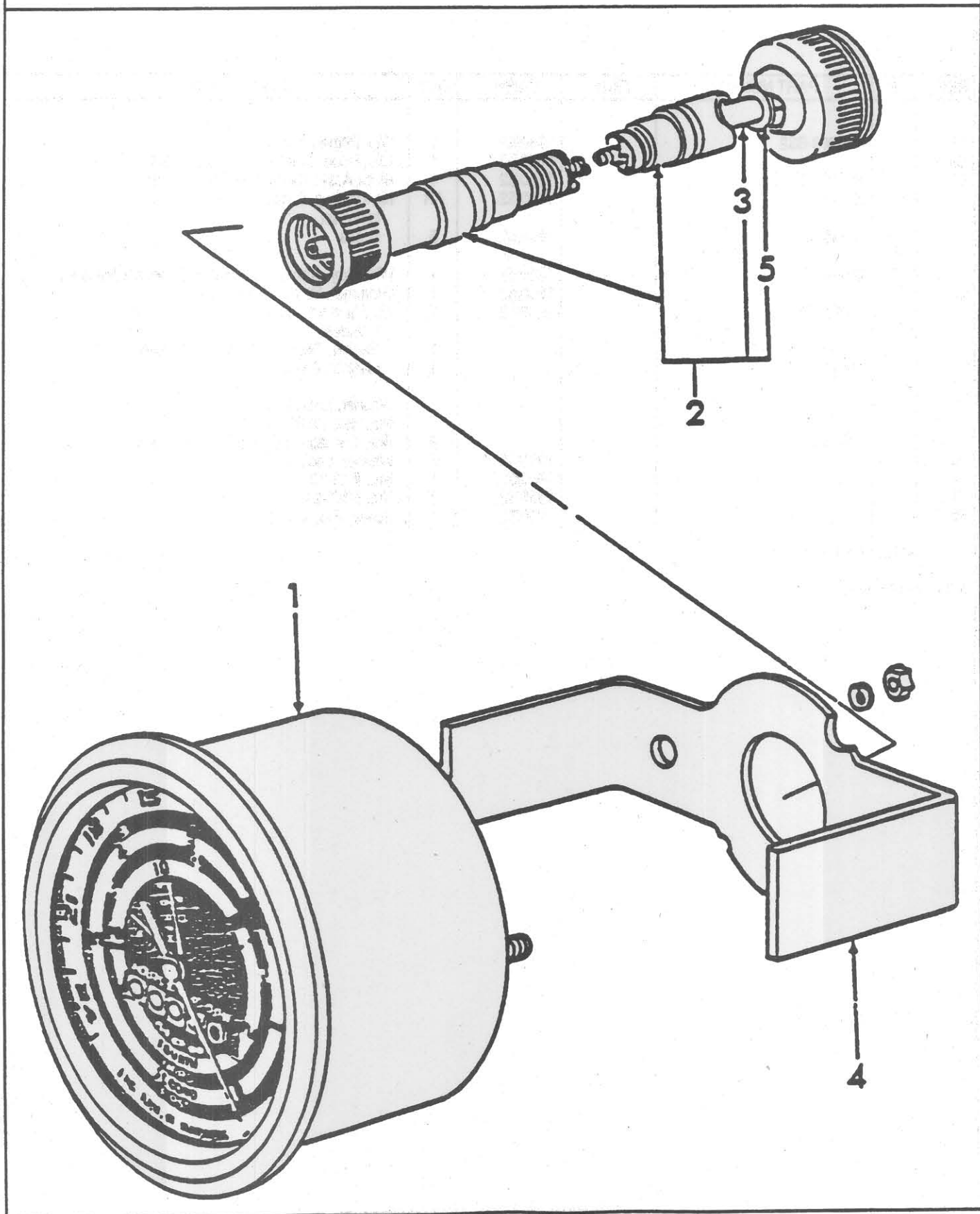
FIG. 12A1 - PROOFMETER &amp; RELATED PARTS - 8N AFTER S/N 290271
