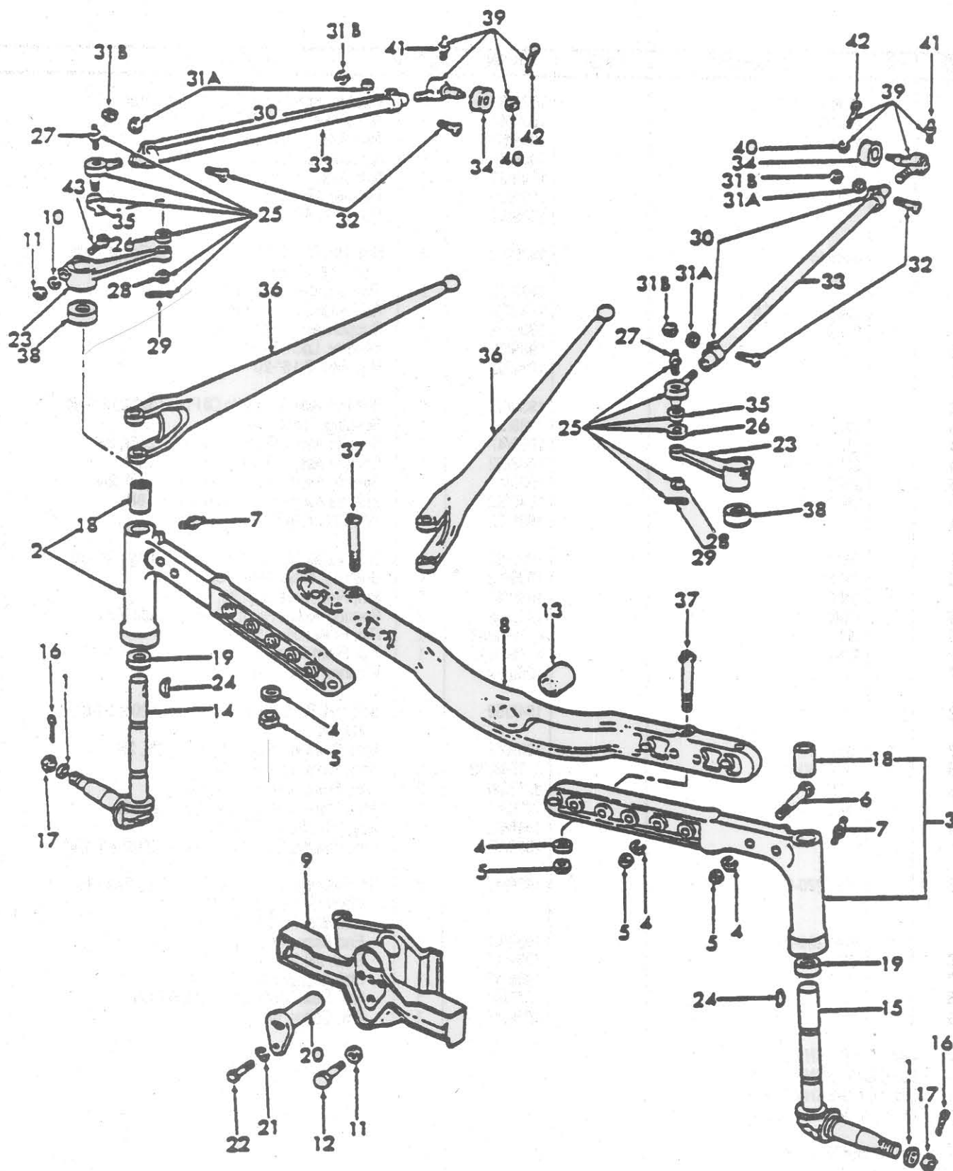
FIG. 3A1 - FRONT AXLE &amp; RELATED PARTS (1939/52) - 9N, 2N, 8N
