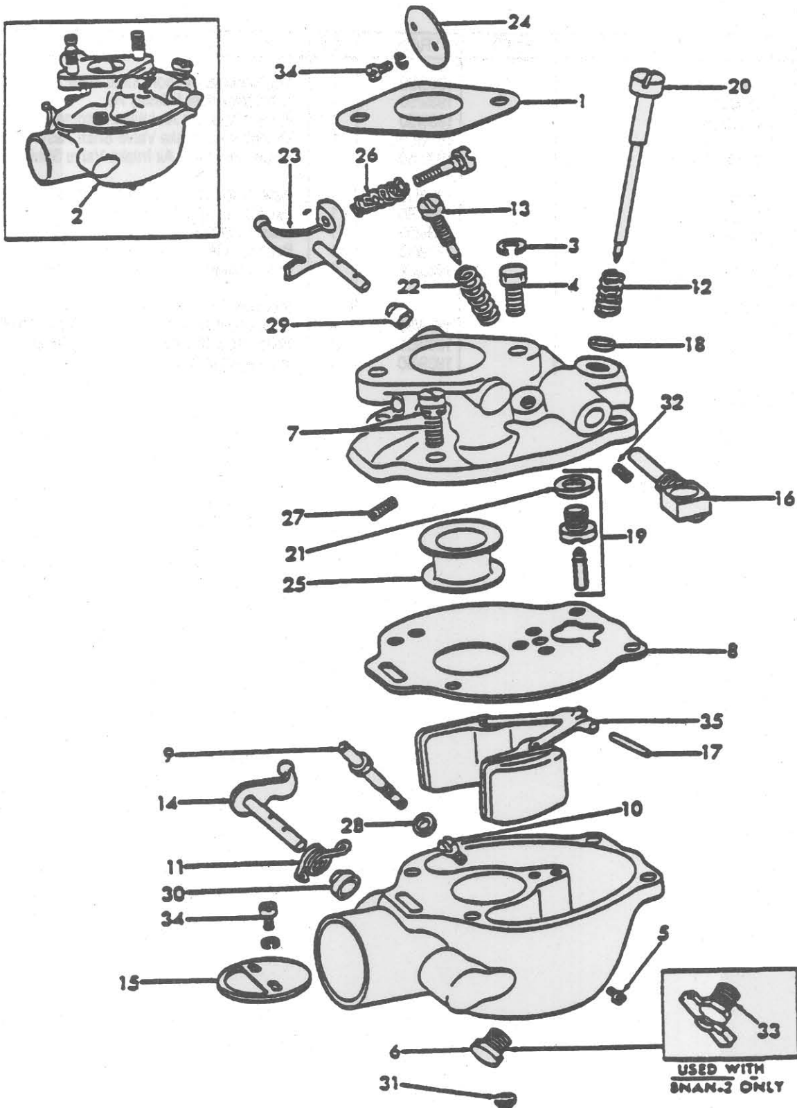
FIG. 9C1 - CARBURETOR ASSY. - 2N, 8N, 9N
