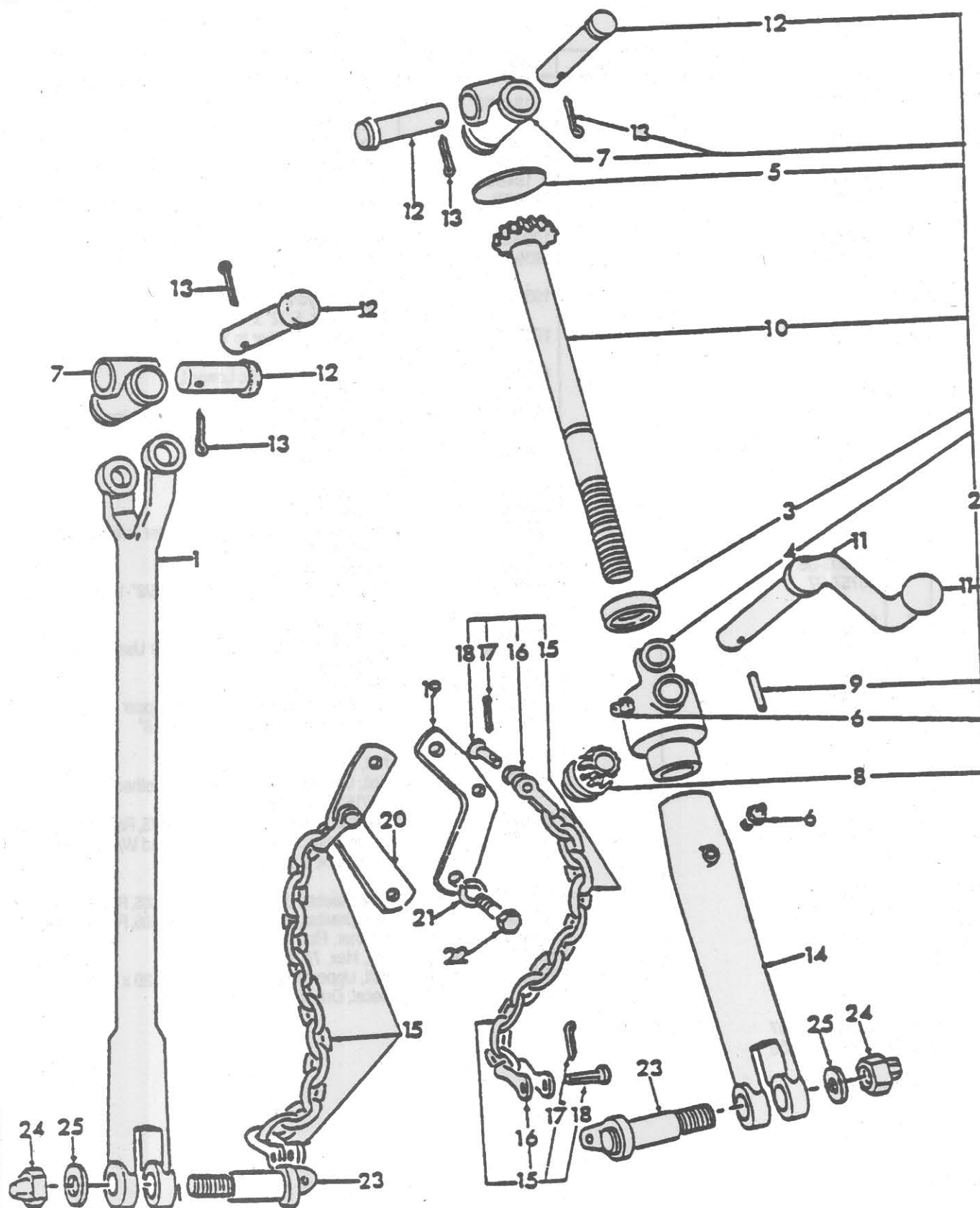
FIG. 5D1 - LEVELING BOX ASSY. &amp; RELATED PARTS - 9N, 2N, 8N
