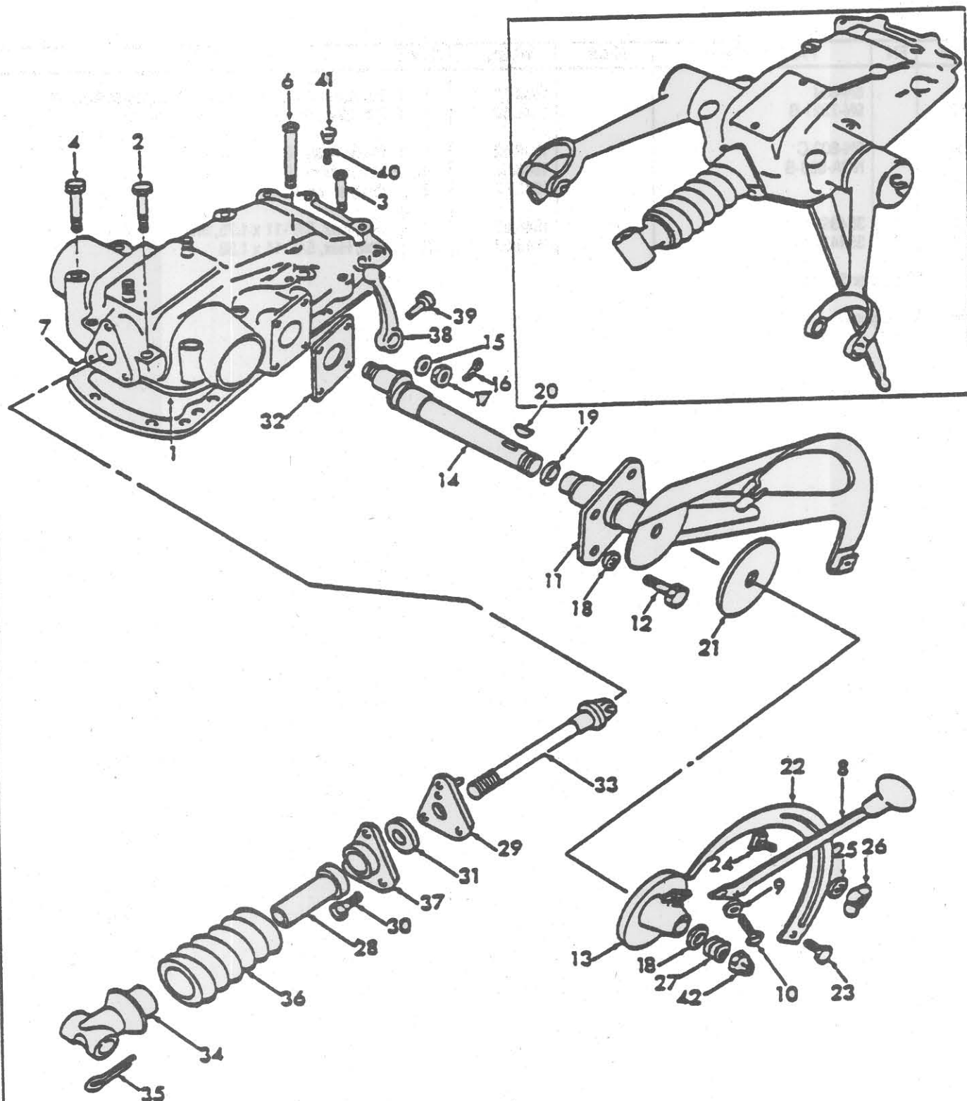
FIG. 5A1 - HYDRAULIC LIFT COVER &amp; RELATED PARTS - 9N, 2N, 8N
