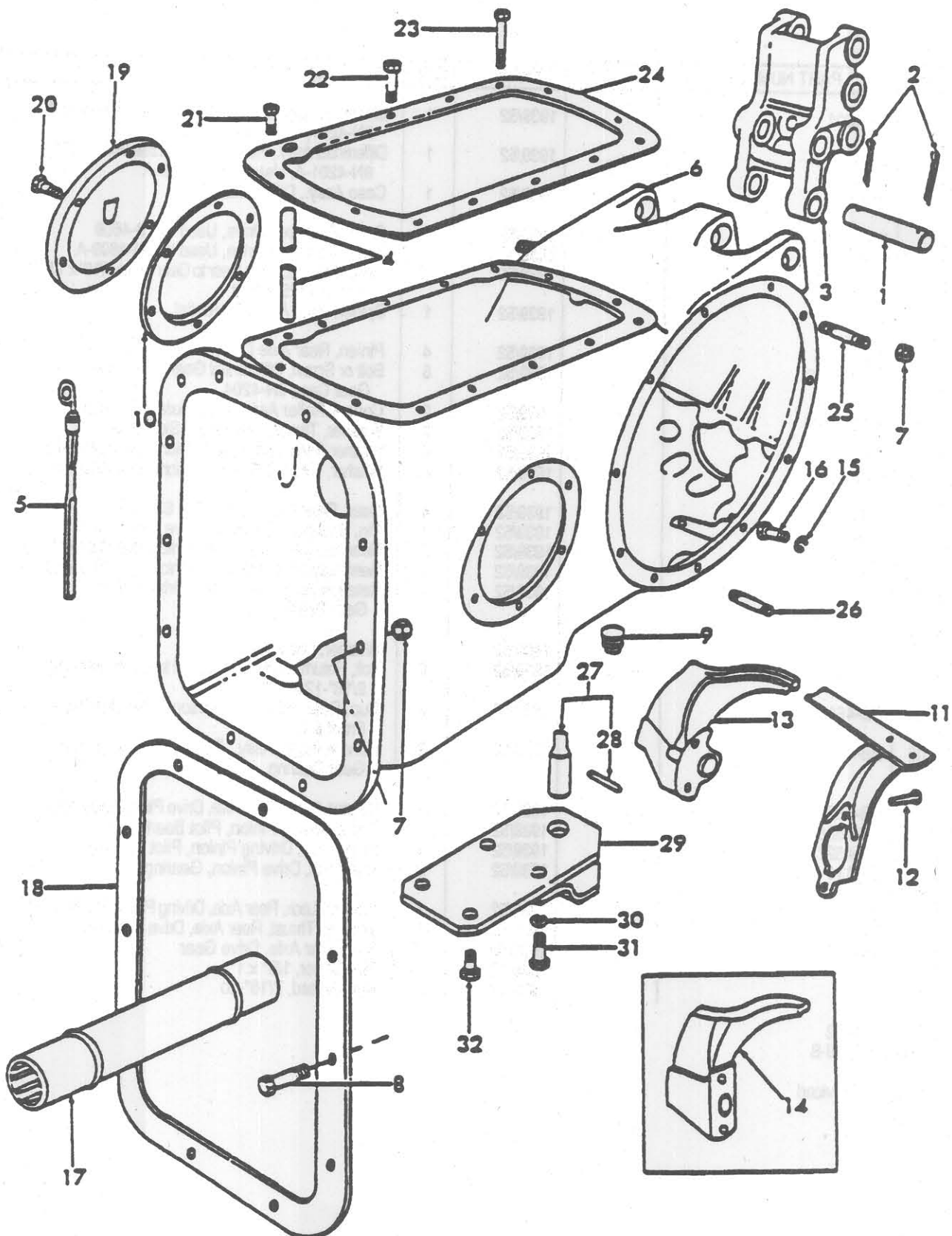
FIG. 4C1 - CENTER HOUSING, ROCKER &amp; RELATED PARTS - 9N, 2N, 8N
