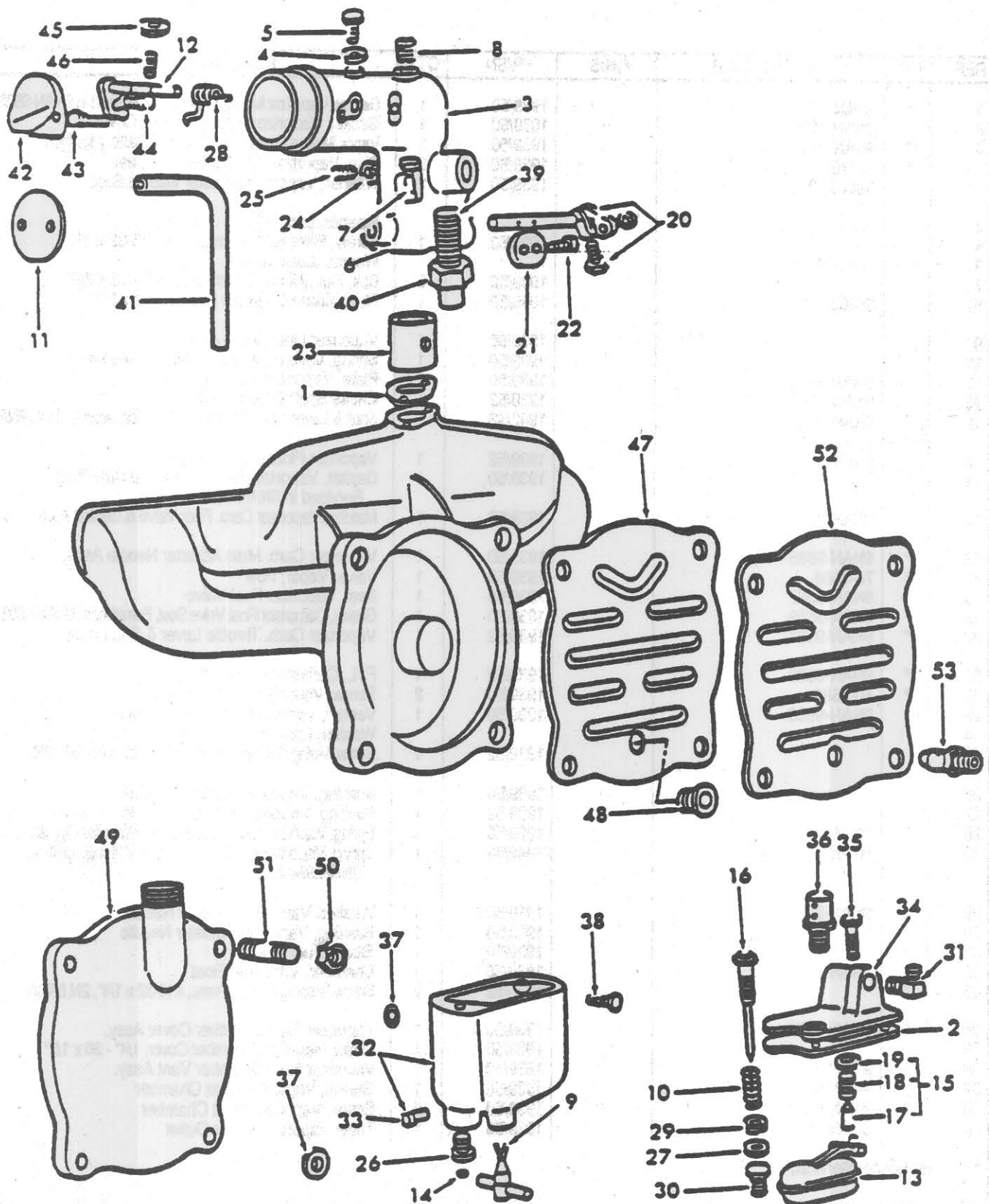
FIG. 9B1 - KEROSENE VAPORIZER ASSY. - 2N, 8N, 9N
