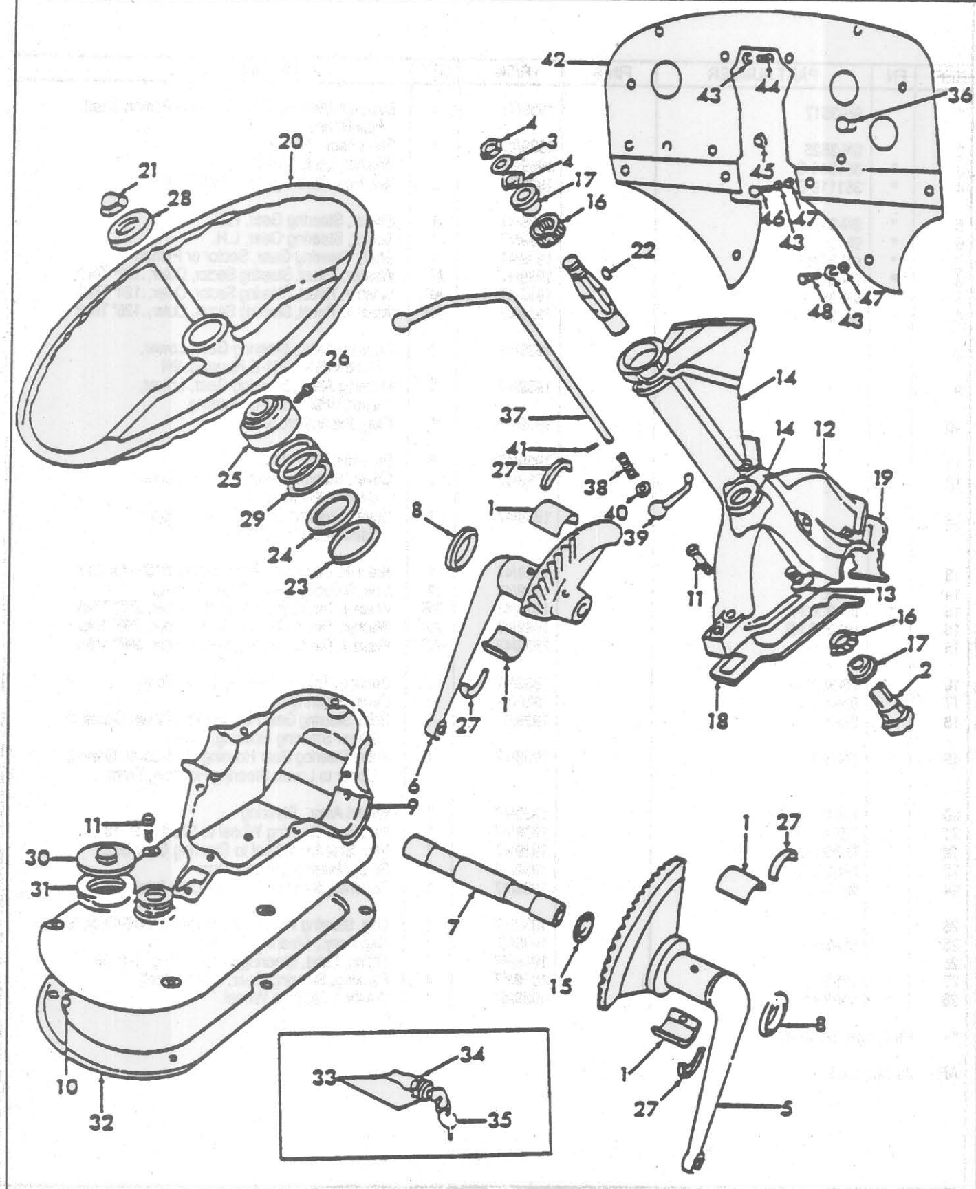
FIG. 3B1 - STEERING GEAR &amp; RELATED PARTS - 9N, 2N
