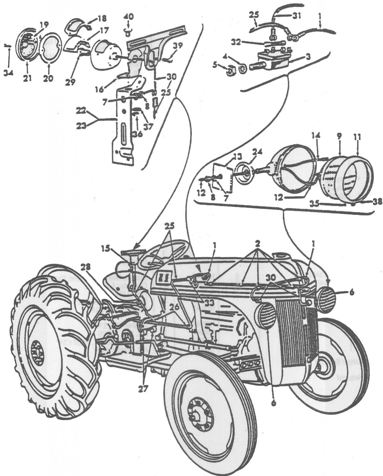
FIG. 11H1 - LIGHTING KIT &amp; WIRING - 8N
