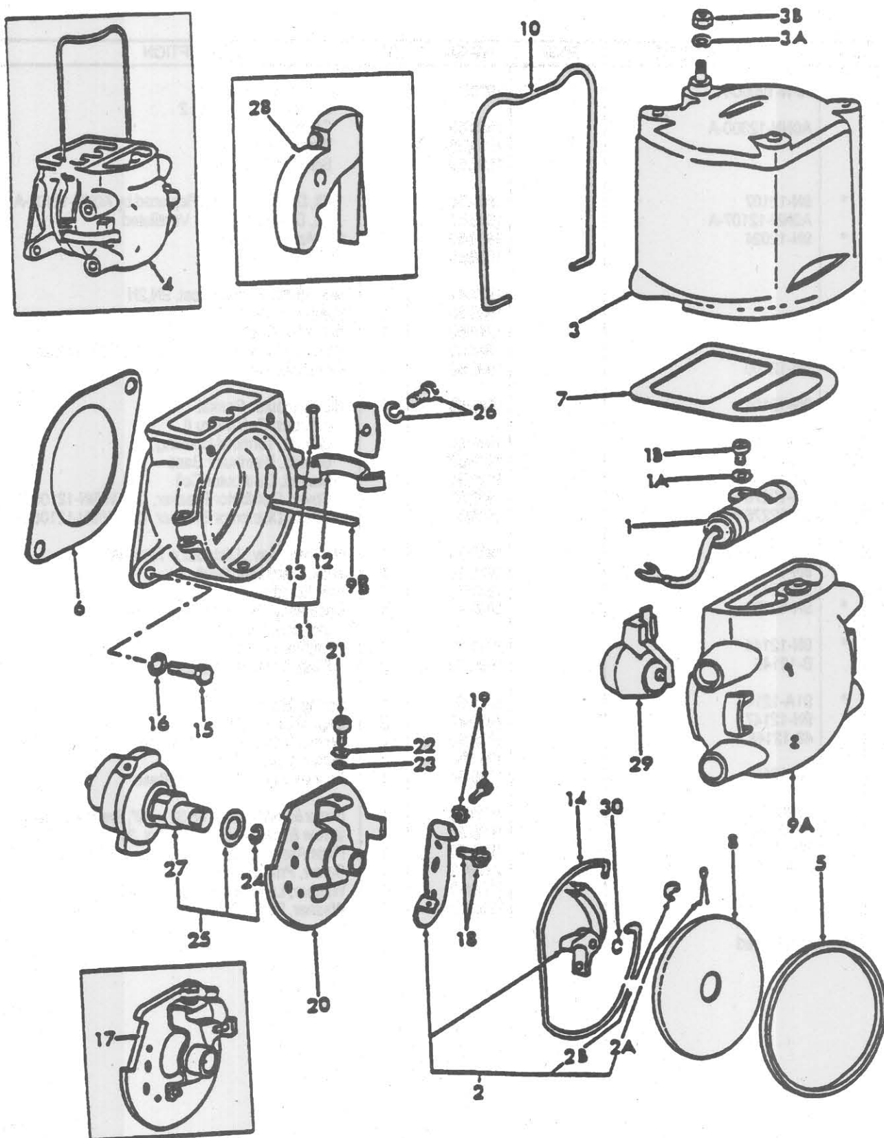
FIG. 11D1 - DISTRIBUTOR & COIL ASSY. - 9N,2N,8N - BEFORE S/N 263844
