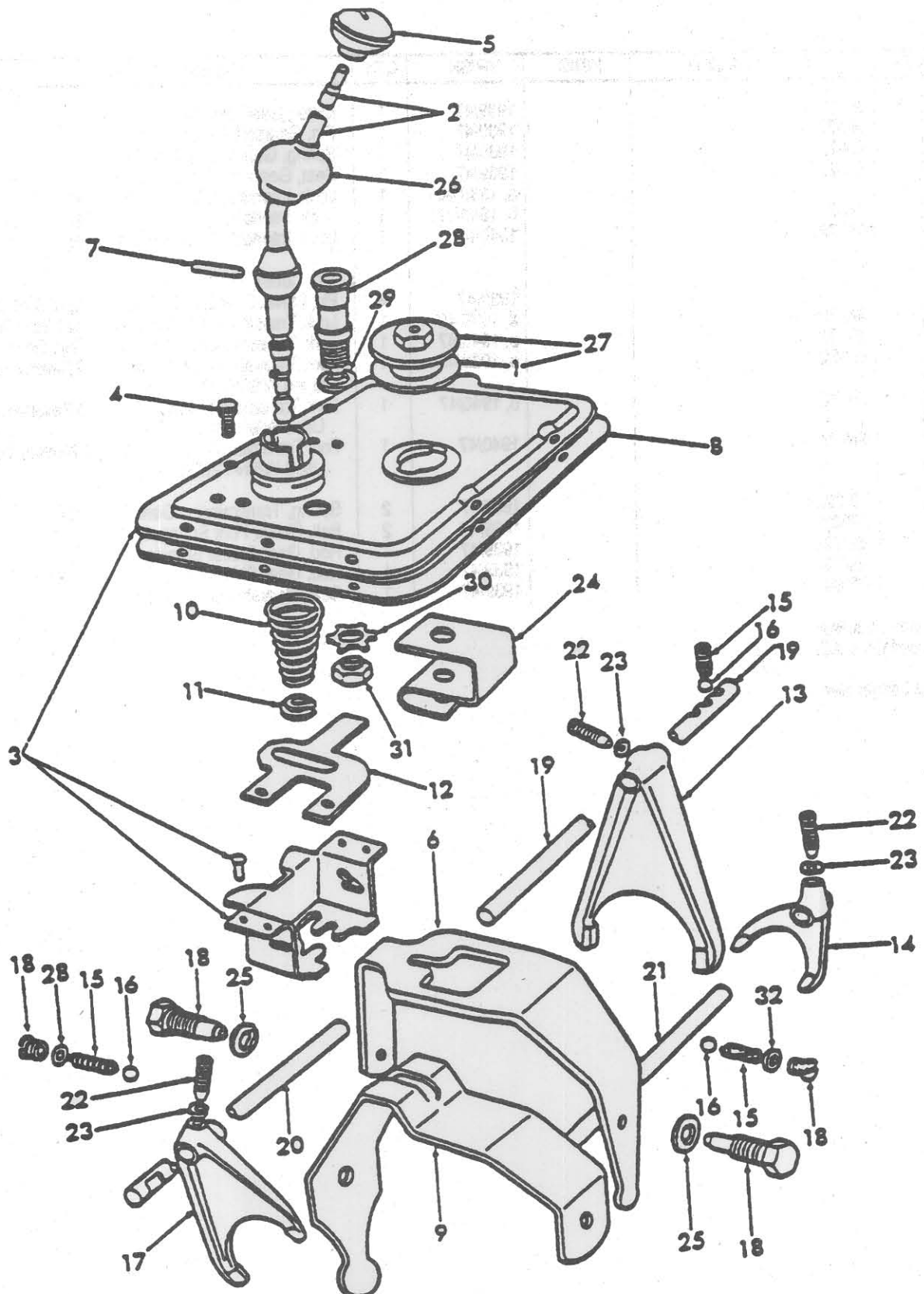
FIG. 7B2 - GEARSHIFT & RELATED PARTS - 8N
