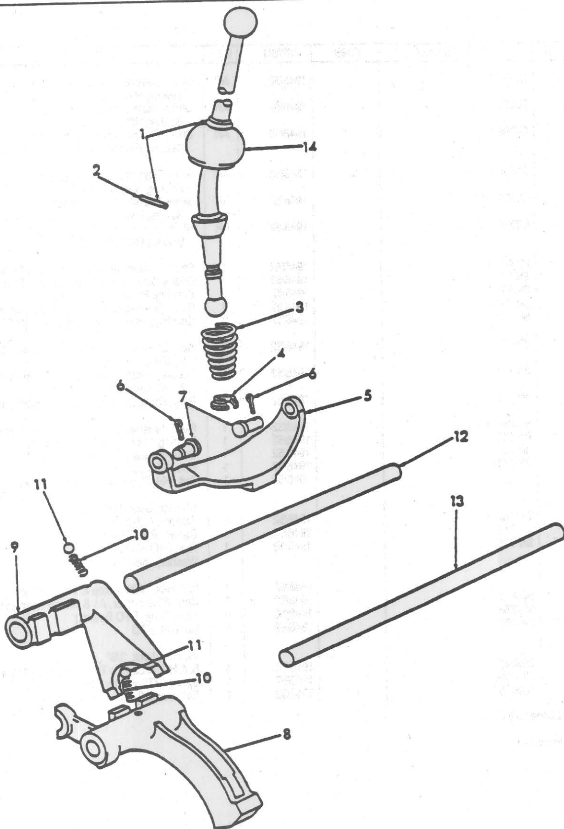
FIG. 7B1 - GEARSHIFT &amp; RELATED PARTS - 9N, 2N
