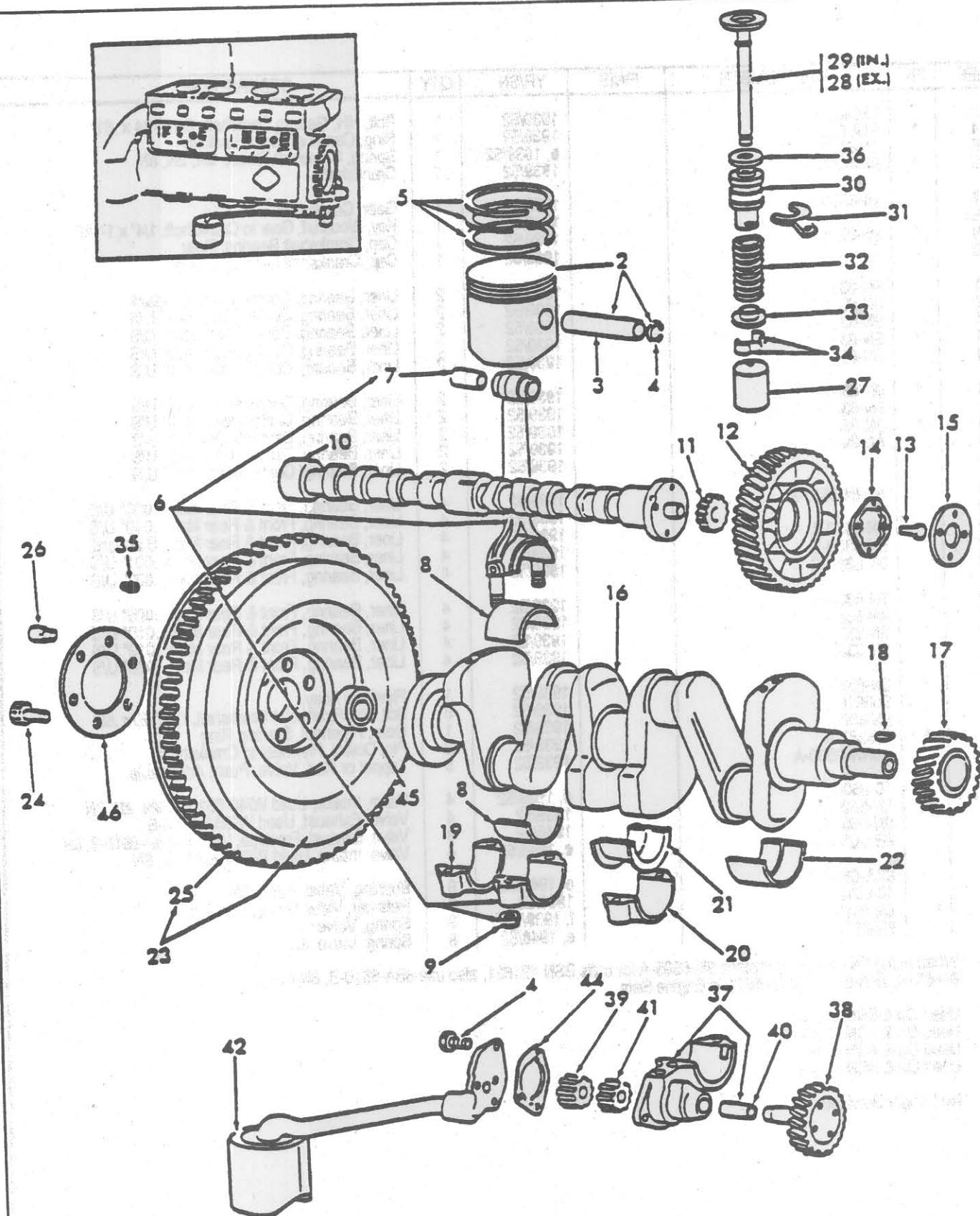
FIG. 6C1 - ENGINE ASSY. (INSIDE) - 9N, 2N, 8N
