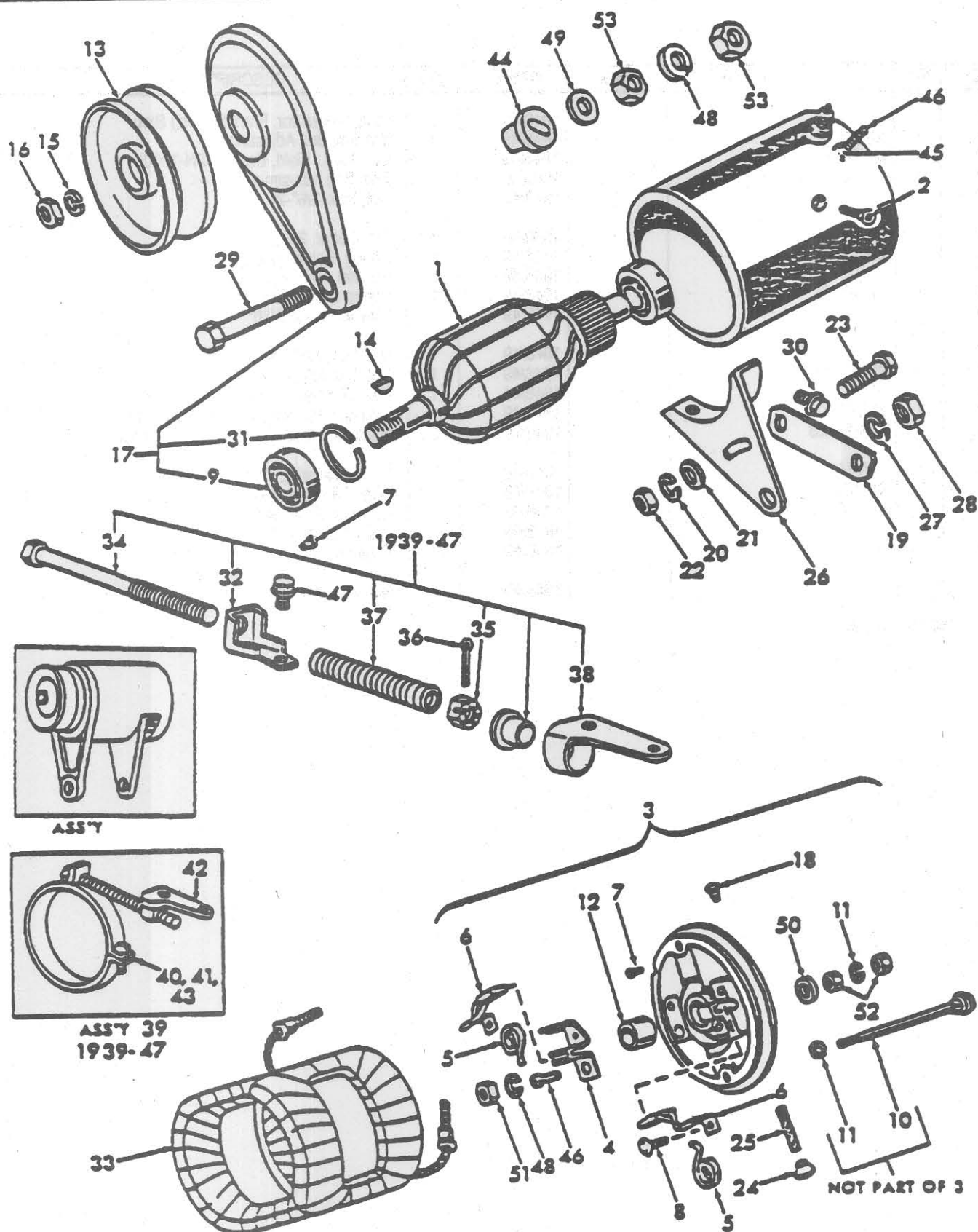
FIG. 11B2 - GENERATOR ASSY. &amp; RELATED PARTS - (2 BRUSH) - 9N,2N
