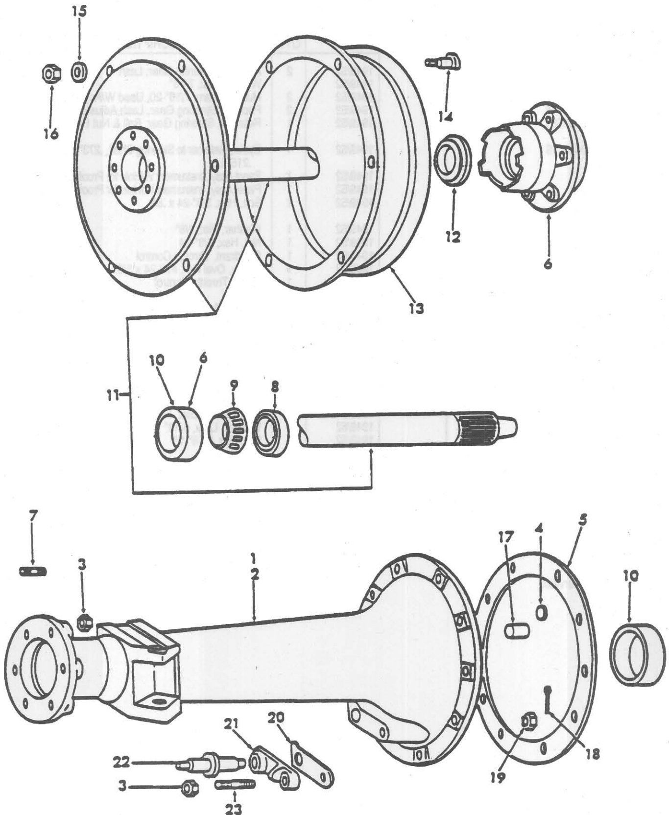
FIG. 4A1 - REAR AXLE SHAFT HOUSING &amp; RELATED PARTS - 9N, 2N
