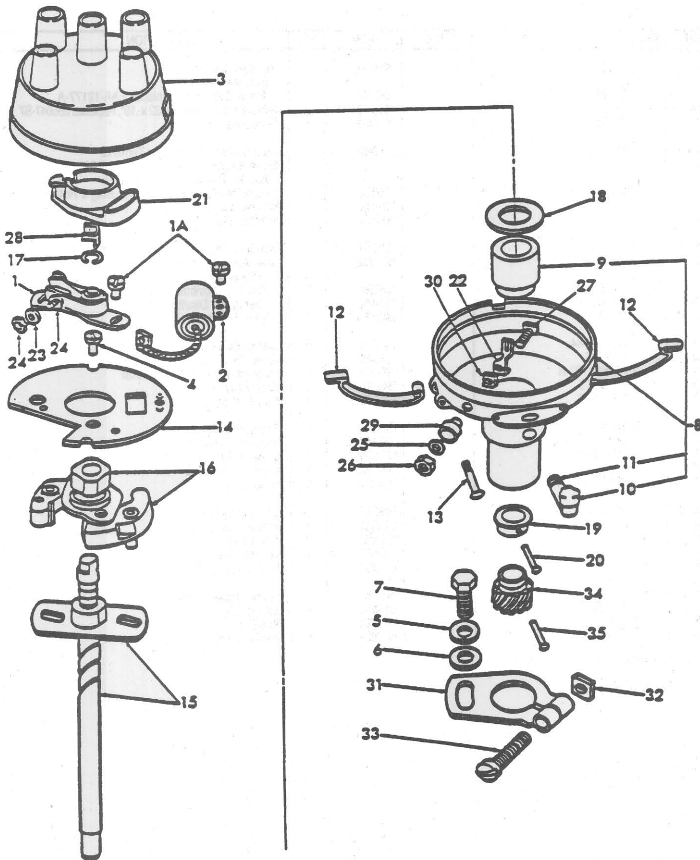
FIG. 11D2 - DISTRIBUTOR - 8N AFTER S/N 263843
