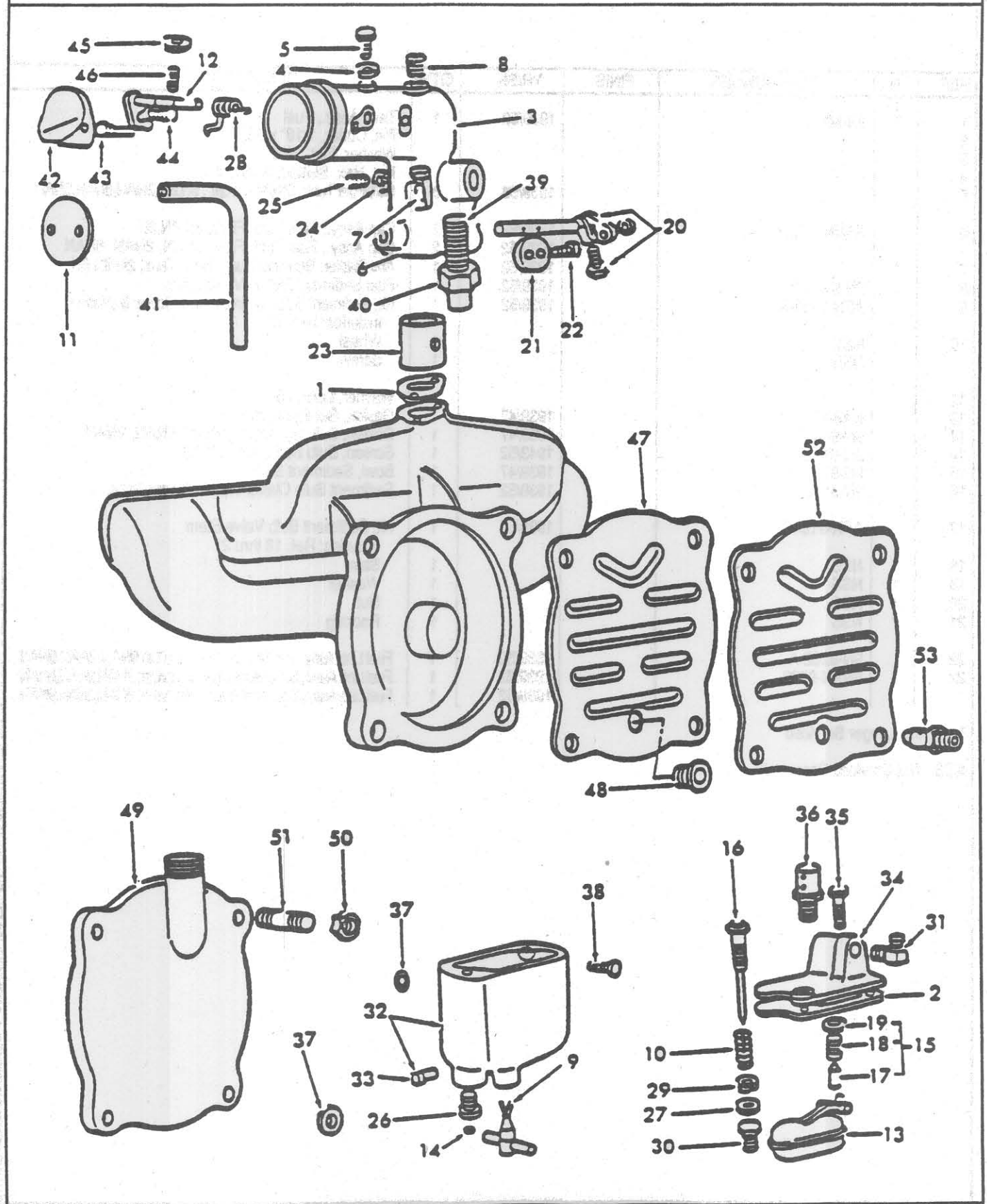
FIG. 9B1 - KEROSENE VAPORIZER ASSY. - 2N, 8N, 9N
